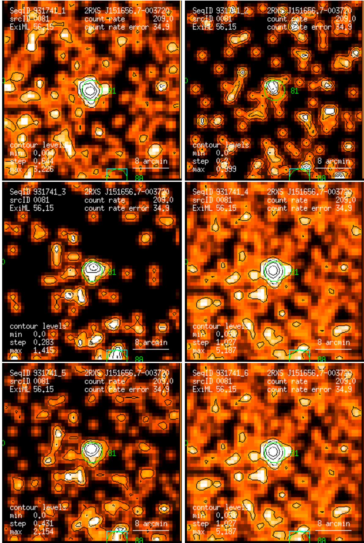
Figure 81: RASS 931741: detection 0081: band rate images, Gaussian filter: (1) PSPC channels 11 – 41, (2) 52 – 90, (3) 91 – 201, (4) 11 – 235, (5) 52 – 201, (6) 11 – 201. Broad band rates in counts/ks. Band rate contour levels in counts/ks/arcmin 2 .
