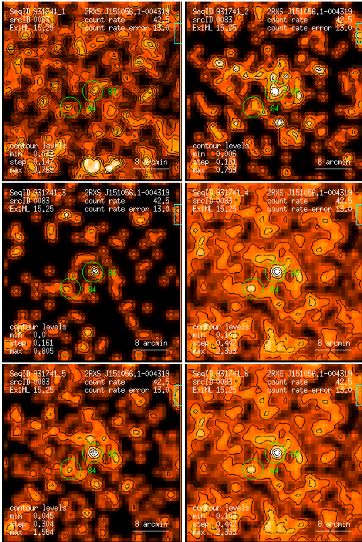
Figure 83: RASS 931741: detection 0083: band rate images, Gaussian filter: (1) PSPC channels 11 – 41, (2) 52 – 90, (3) 91 – 201, (4) 11 – 235, (5) 52 – 201, (6) 11 – 201. Broad band rates in counts/ks. Band rate contour levels in counts/ks/arcmin 2 .
