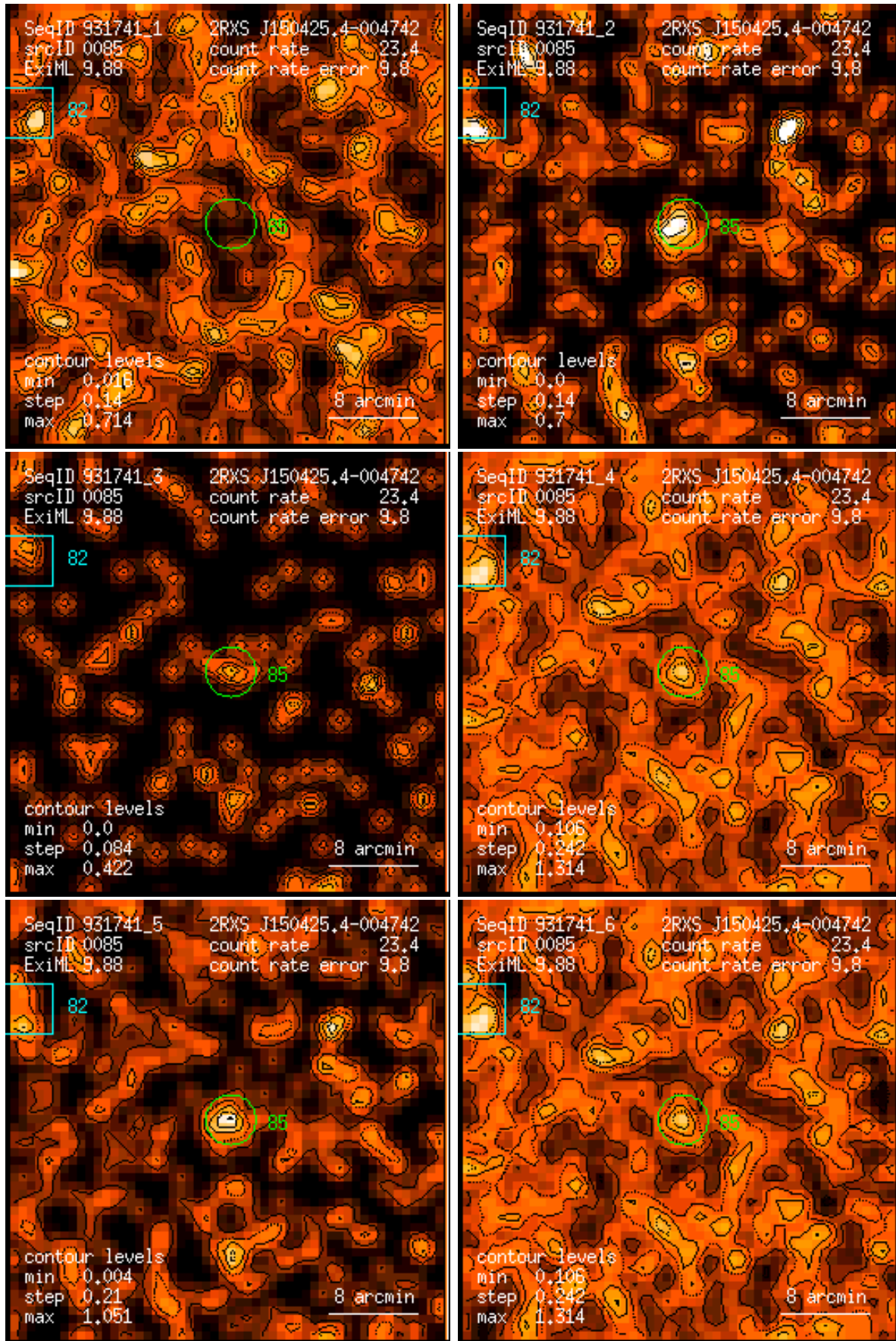
Figure 85: RASS 931741: detection 0085: band rate images, Gaussian filter: (1) PSPC channels 11 – 41, (2) 52 – 90, (3) 91 – 201, (4) 11 – 235, (5) 52 – 201, (6) 11 – 201. Broad band rates in counts/ks. Band rate contour levels in counts/ks/arcmin 2 .
