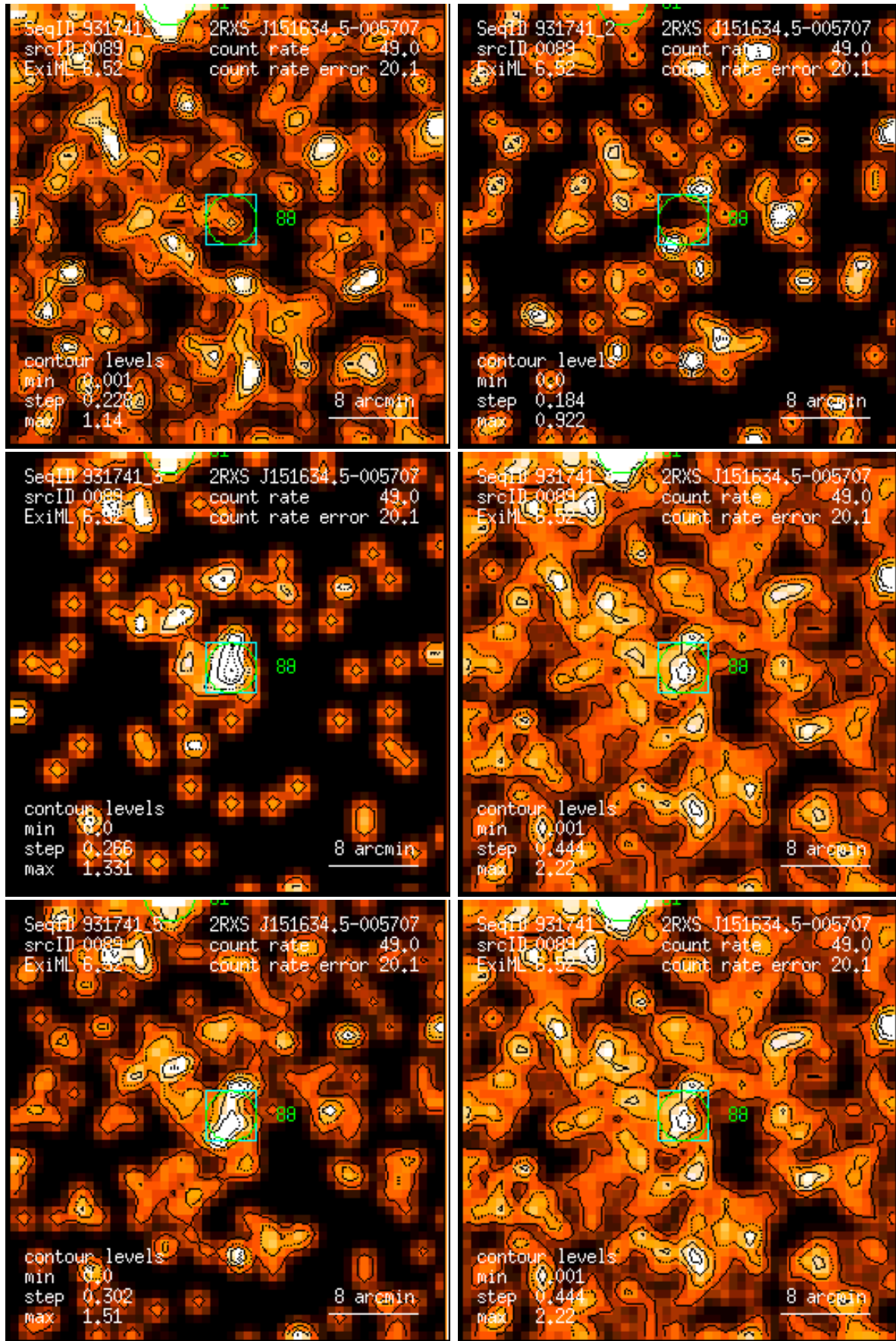
Figure 89: RASS 931741: detection 0089: band rate images, Gaussian filter: (1) PSPC channels 11 – 41, (2) 52 – 90, (3) 91 – 201, (4) 11 – 235, (5) 52 – 201, (6) 11 – 201. Broad band rates in counts/ks. Band rate contour levels in counts/ks/arcmin 2 .
