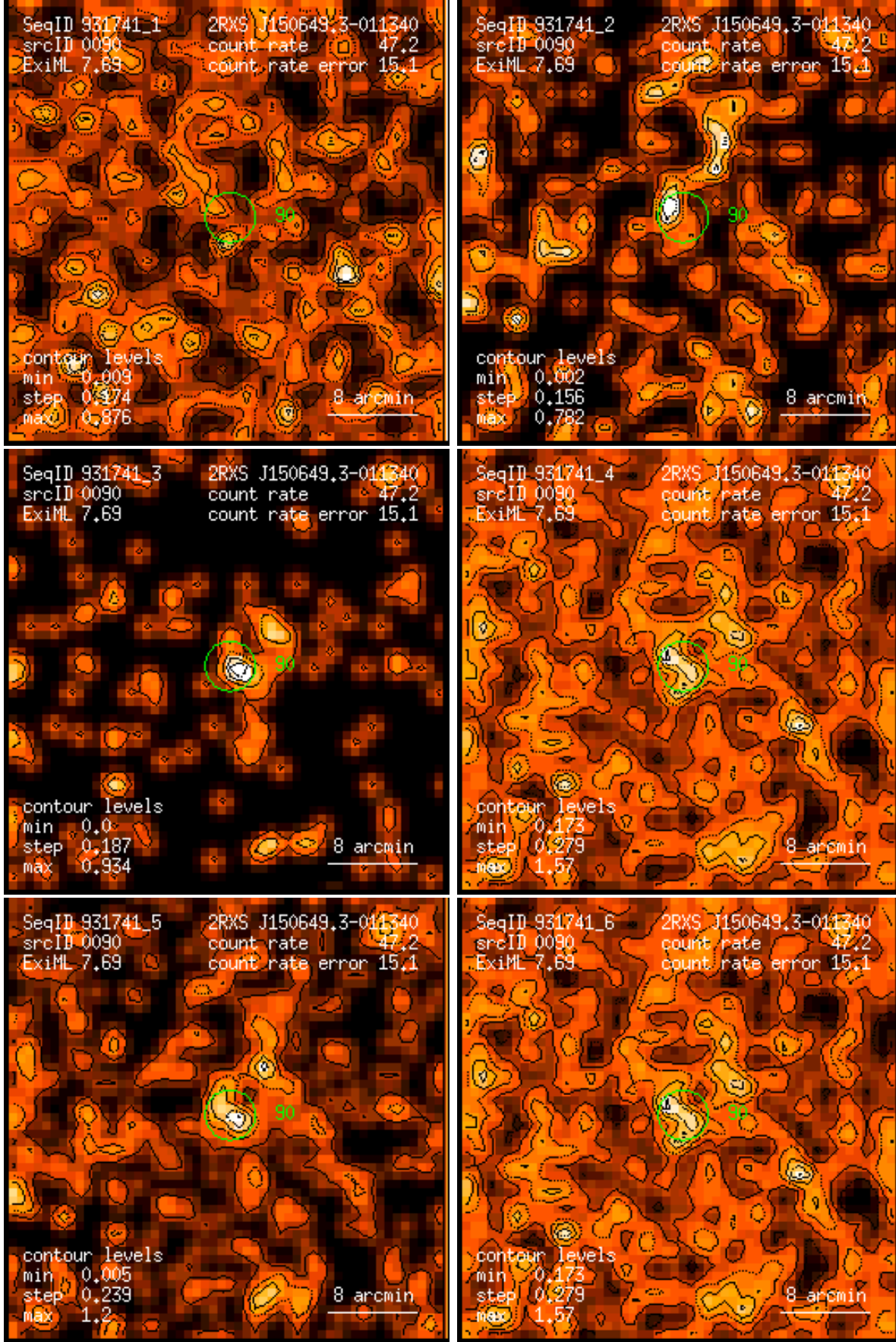
Figure 90: RASS 931741: detection 0090: band rate images, Gaussian filter: (1) PSPC channels 11 – 41, (2) 52 – 90, (3) 91 – 201, (4) 11 – 235, (5) 52 – 201, (6) 11 – 201. Broad band rates in counts/ks. Band rate contour levels in counts/ks/arcmin 2 .
