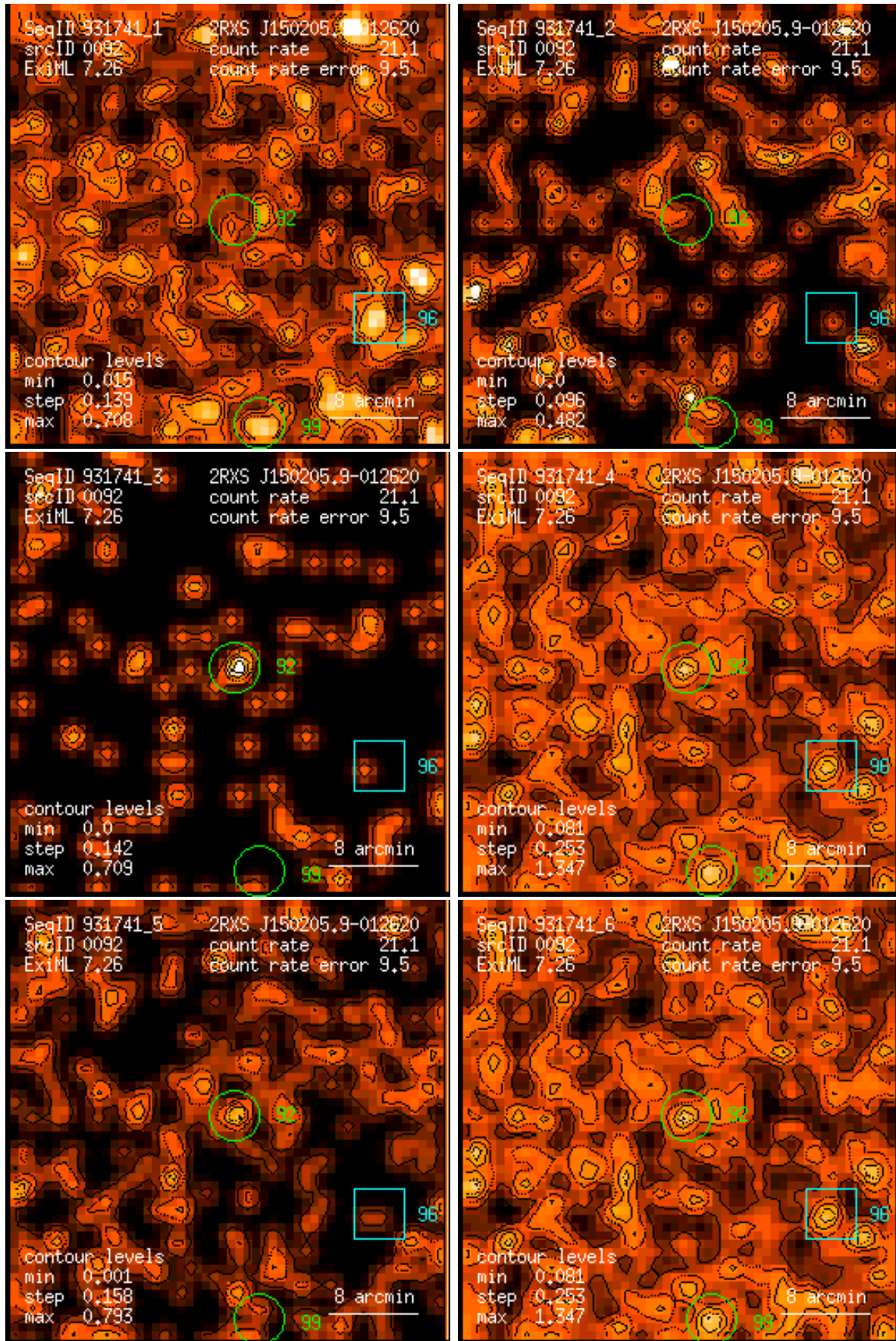
Figure 92: RASS 931741: detection 0092: band rate images, Gaussian filter: (1) PSPC channels 11 – 41, (2) 52 – 90, (3) 91 – 201, (4) 11 – 235, (5) 52 – 201, (6) 11 – 201. Broad band rates in counts/ks. Band rate contour levels in counts/ks/arcmin 2 .
