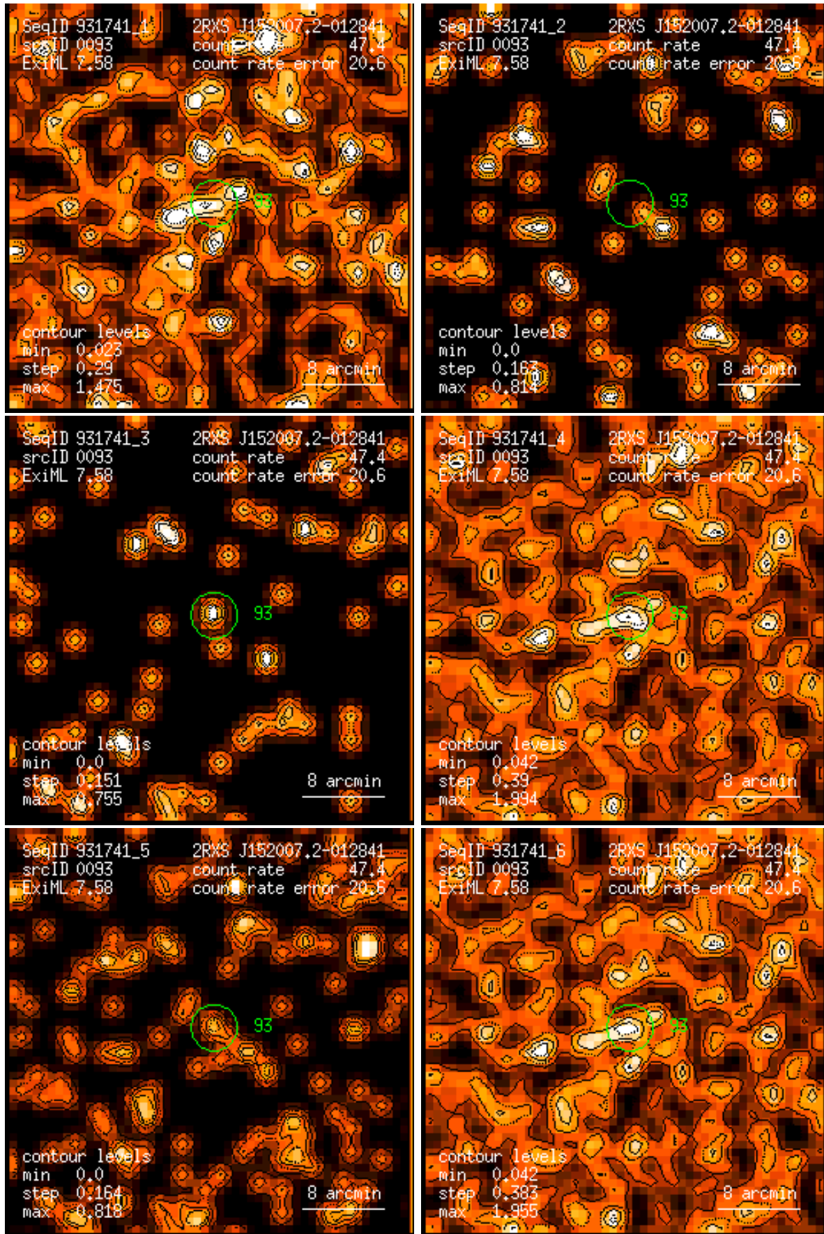
Figure 93: RASS 931741: detection 0093: band rate images, Gaussian filter: (1) PSPC channels 11 – 41, (2) 52 – 90, (3) 91 – 201, (4) 11 – 235, (5) 52 – 201, (6) 11 – 201. Broad band rates in counts/ks. Band rate contour levels in counts/ks/arcmin 2 .
