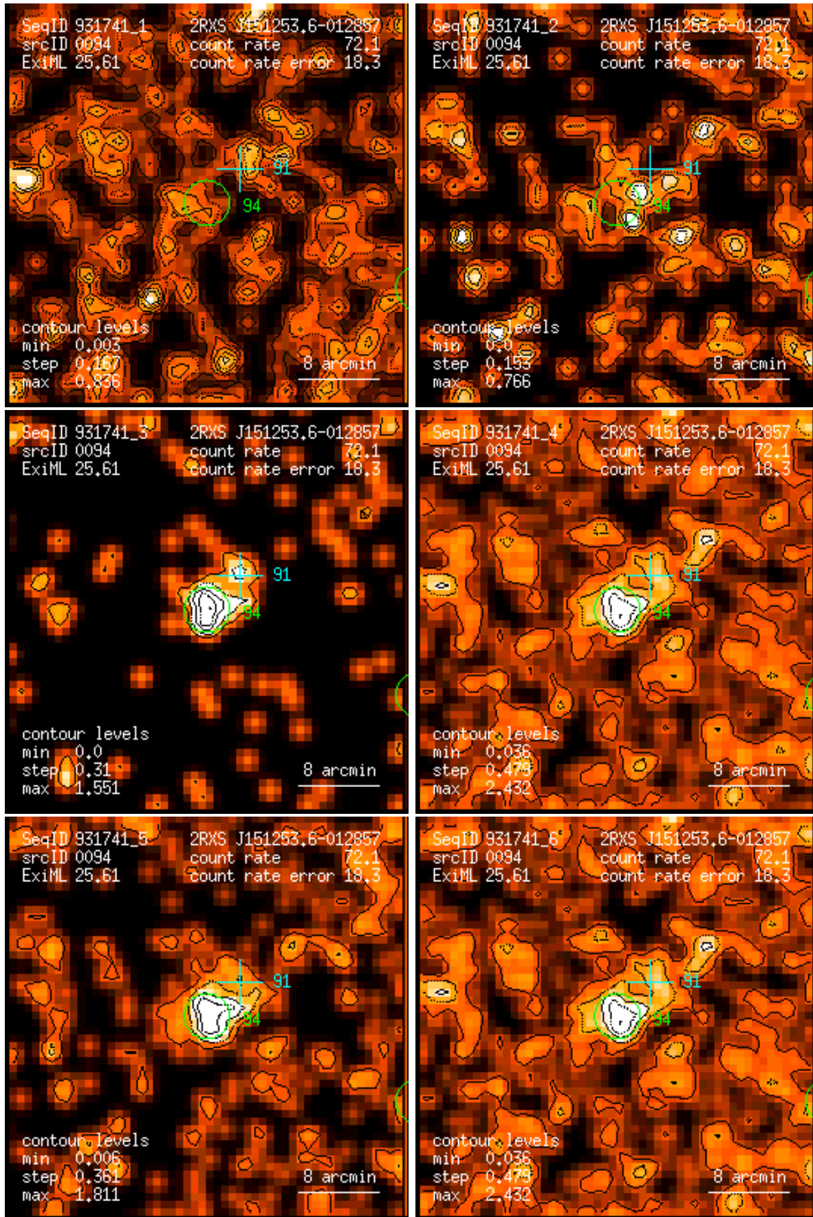
Figure 94: RASS 931741: detection 0094: band rate images, Gaussian filter: (1) PSPC channels 11 – 41, (2) 52 – 90, (3) 91 – 201, (4) 11 – 235, (5) 52 – 201, (6) 11 – 201. Broad band rates in counts/ks. Band rate contour levels in counts/ks/arcmin 2 .
