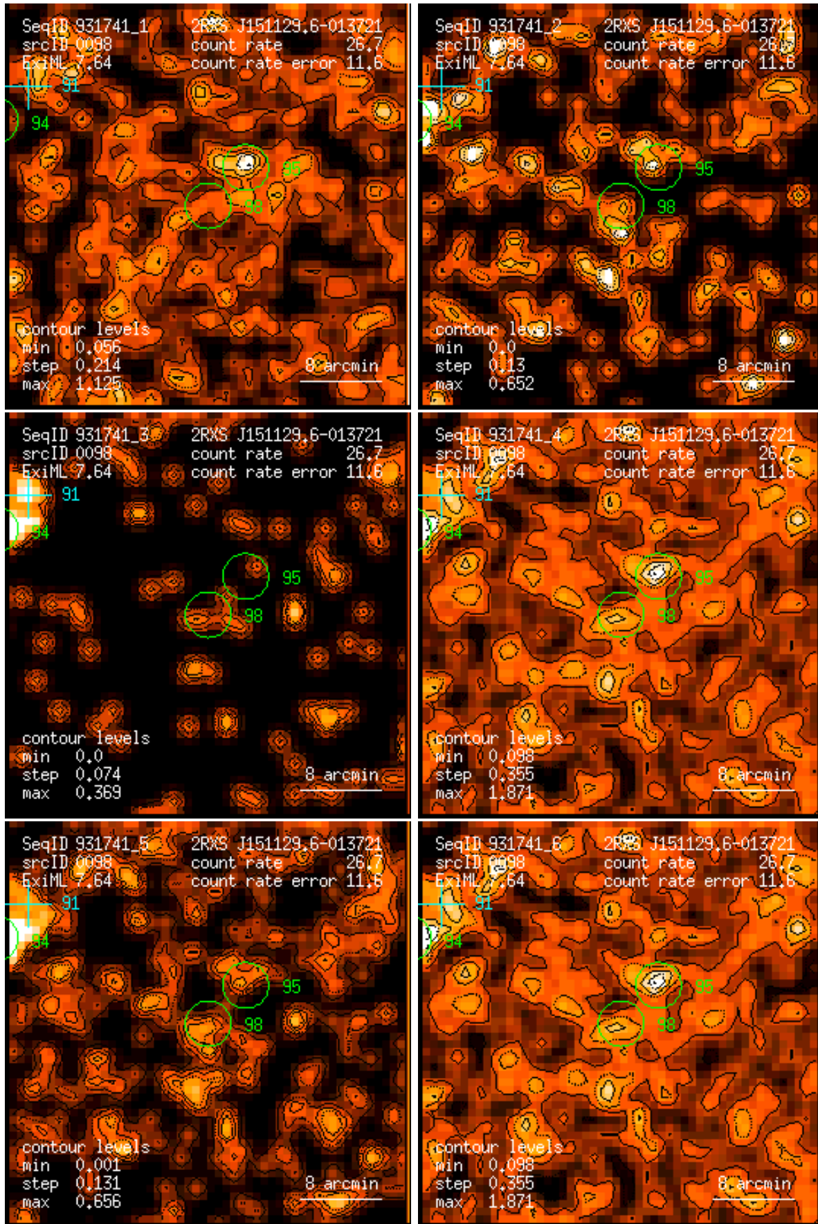
Figure 98: RASS 931741: detection 0098: band rate images, Gaussian filter: (1) PSPC channels 11 – 41, (2) 52 – 90, (3) 91 – 201, (4) 11 – 235, (5) 52 – 201, (6) 11 – 201. Broad band rates in counts/ks. Band rate contour levels in counts/ks/arcmin 2 .
