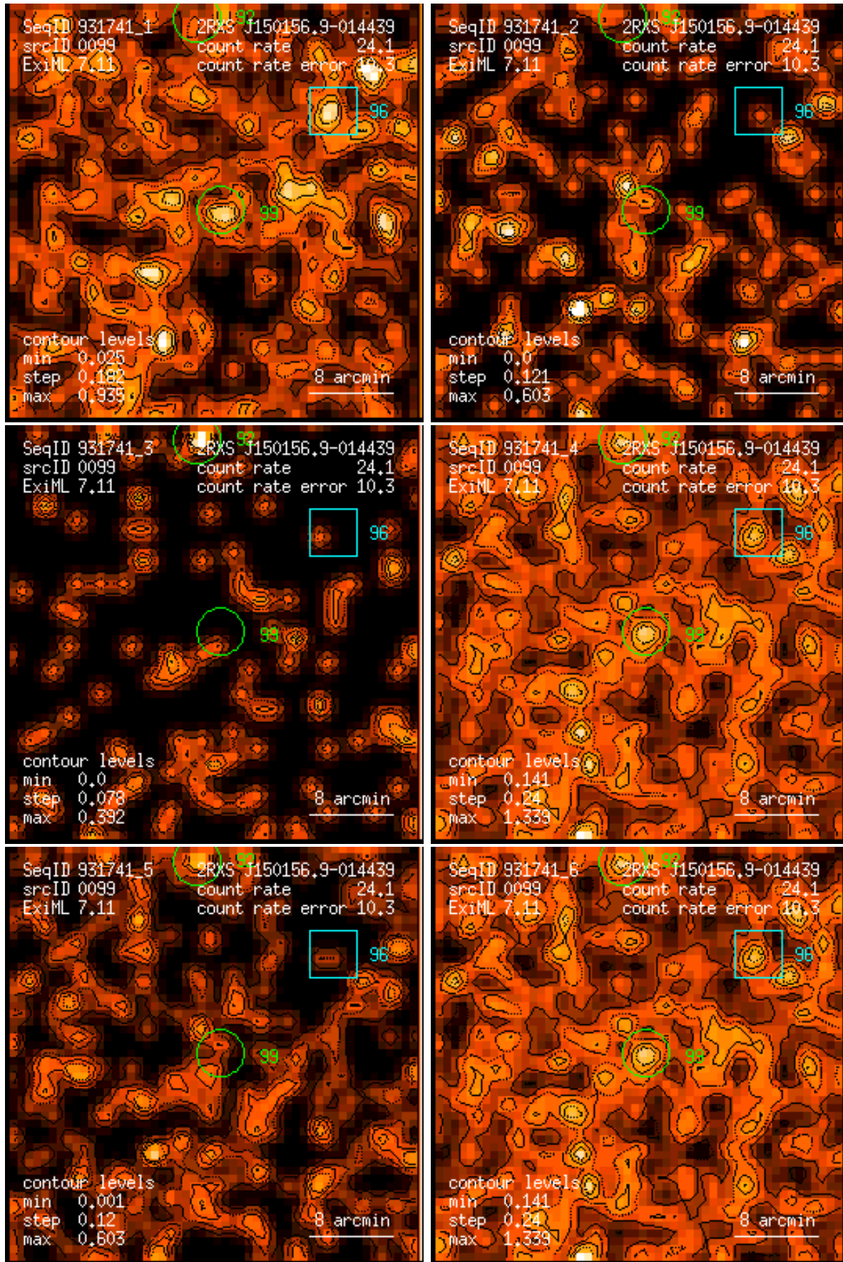
Figure 99: RASS 931741: detection 0099: band rate images, Gaussian filter: (1) PSPC channels 11 – 41, (2) 52 – 90, (3) 91 – 201, (4) 11 – 235, (5) 52 – 201, (6) 11 – 201. Broad band rates in counts/ks. Band rate contour levels in counts/ks/arcmin 2 .
