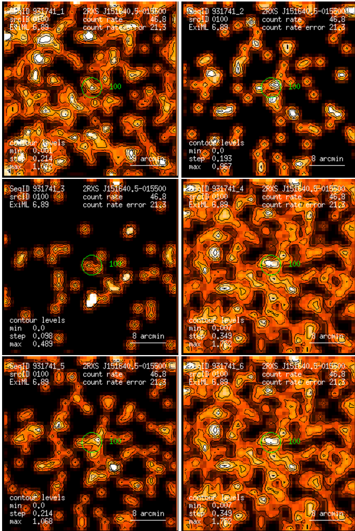
Figure 100: RASS 931741: detection 0100: band rate images, Gaussian filter: (1) PSPC channels 11 – 41, (2) 52 – 90, (3) 91 – 201, (4) 11 – 235, (5) 52 – 201, (6) 11 – 201. Broad band rates in counts/ks. Band rate contour levels in counts/ks/arcmin 2 .
