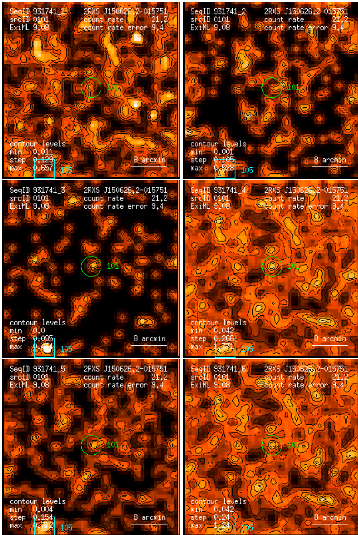
Figure 101: RASS 931741: detection 0101: band rate images, Gaussian filter: (1) PSPC channels 11 – 41, (2) 52 – 90, (3) 91 – 201, (4) 11 – 235, (5) 52 – 201, (6) 11 – 201. Broad band rates in counts/ks. Band rate contour levels in counts/ks/arcmin 2 .
