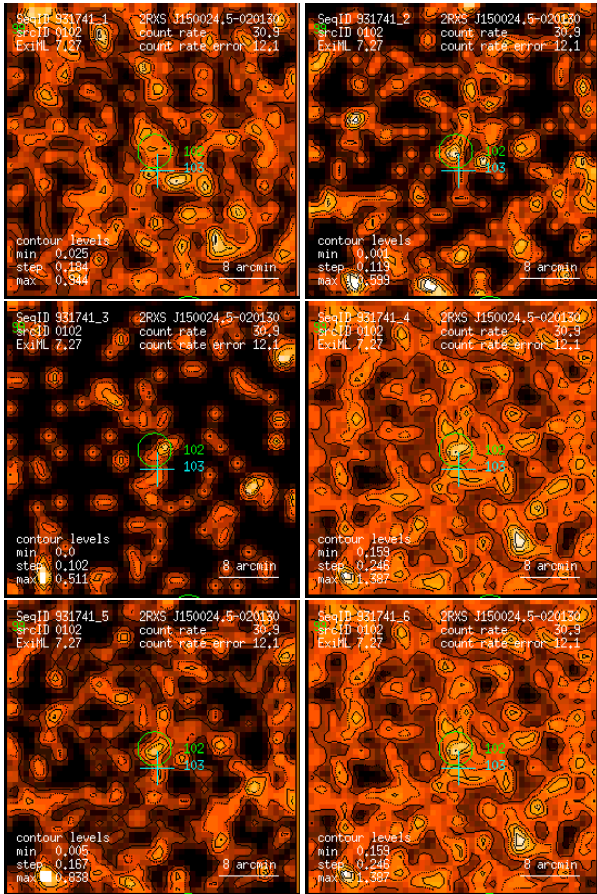
Figure 102: RASS 931741: detection 0102: band rate images, Gaussian filter: (1) PSPC channels 11 – 41, (2) 52 – 90, (3) 91 – 201, (4) 11 – 235, (5) 52 – 201, (6) 11 – 201. Broad band rates in counts/ks. Band rate contour levels in counts/ks/arcmin 2 .
