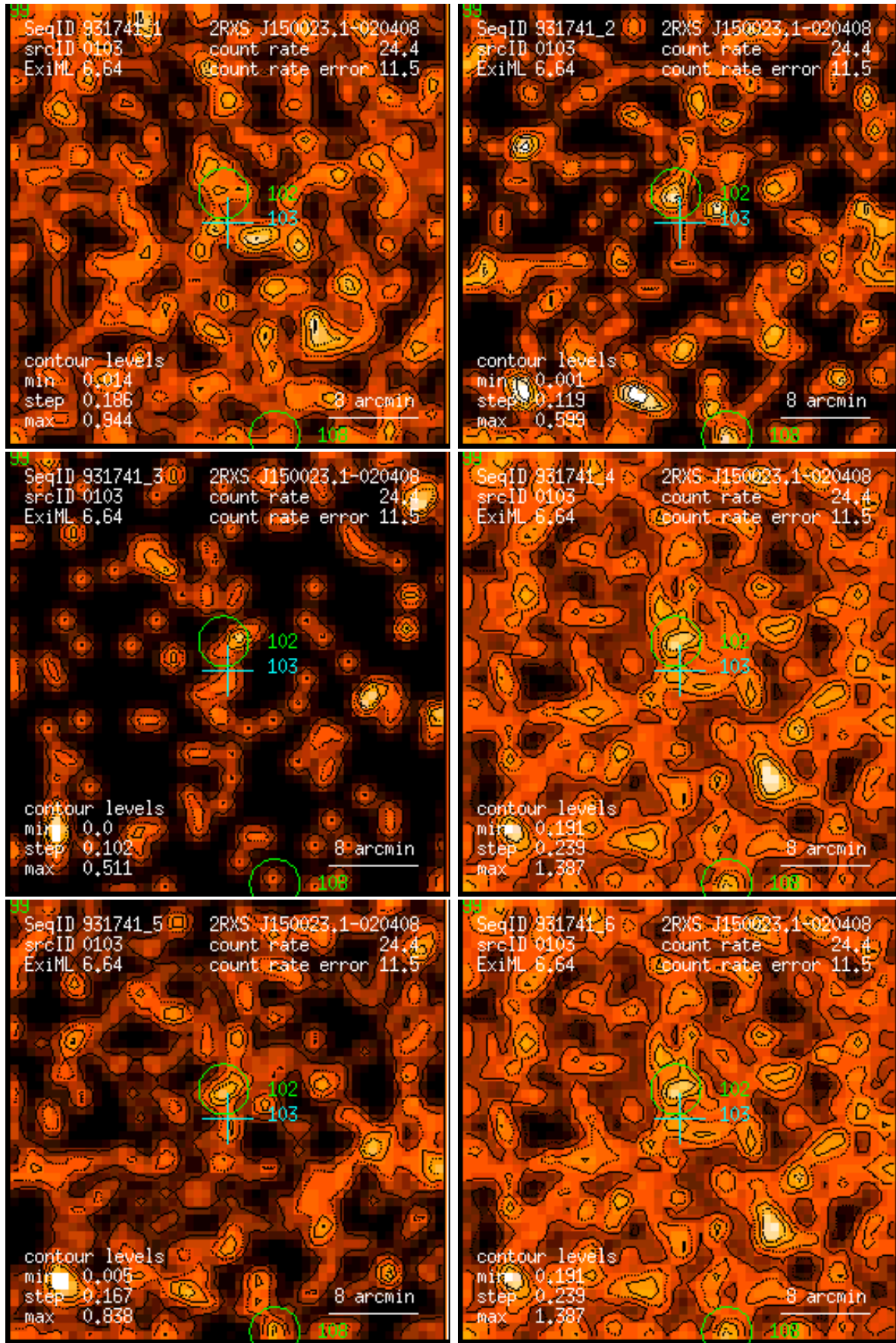
Figure 103: RASS 931741: detection 0103: band rate images, Gaussian filter: (1) PSPC channels 11 – 41, (2) 52 – 90, (3) 91 – 201, (4) 11 – 235, (5) 52 – 201, (6) 11 – 201. Broad band rates in counts/ks. Band rate contour levels in counts/ks/arcmin 2 .
