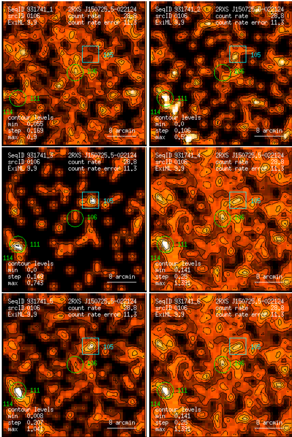
Figure 106: RASS 931741: detection 0106: band rate images, Gaussian filter: (1) PSPC channels 11 – 41, (2) 52 – 90, (3) 91 – 201, (4) 11 – 235, (5) 52 – 201, (6) 11 – 201. Broad band rates in counts/ks. Band rate contour levels in counts/ks/arcmin 2 .
