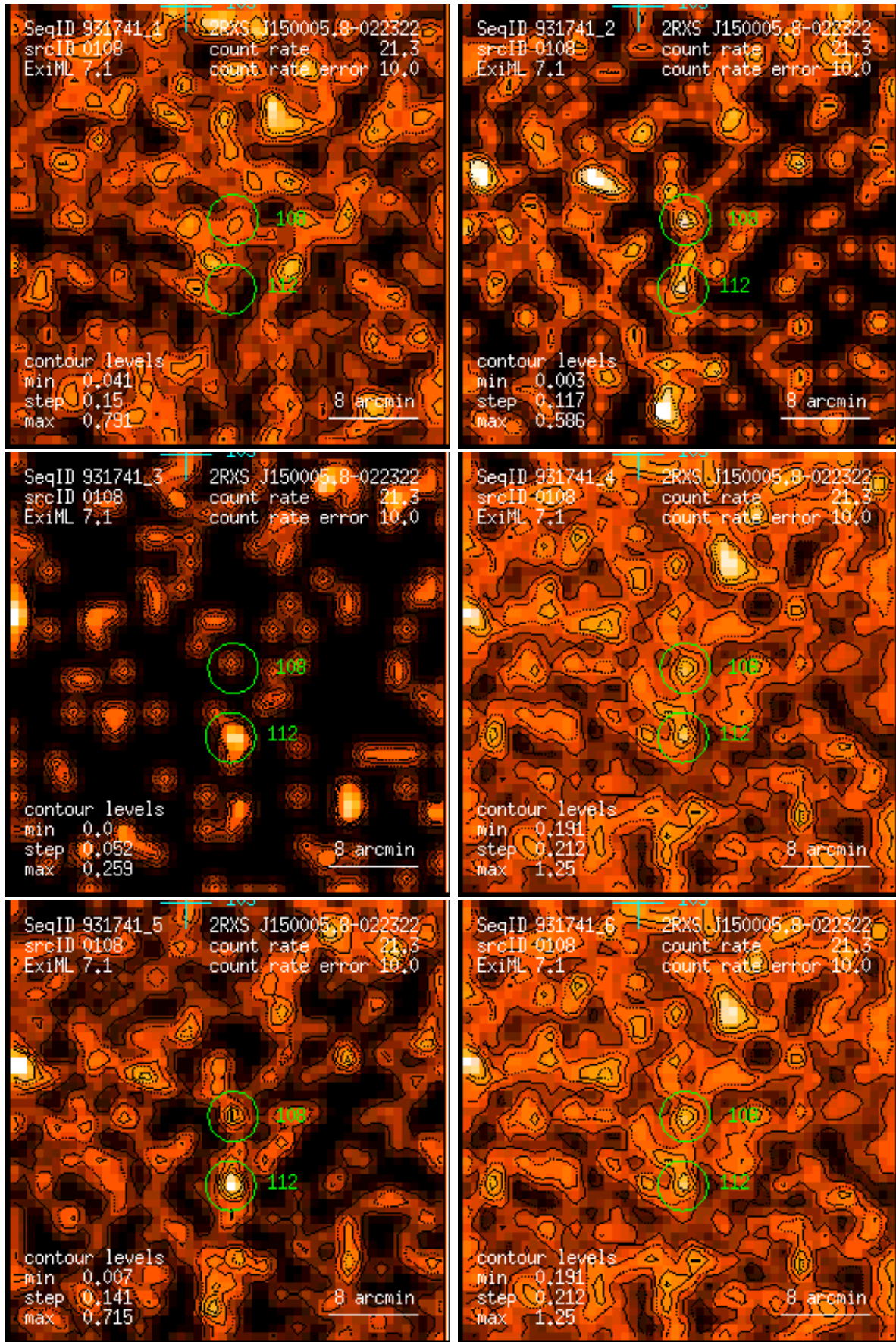
Figure 108: RASS 931741: detection 0108: band rate images, Gaussian filter: (1) PSPC channels 11 – 41, (2) 52 – 90, (3) 91 – 201, (4) 11 – 235, (5) 52 – 201, (6) 11 – 201. Broad band rates in counts/ks. Band rate contour levels in counts/ks/arcmin 2 .
