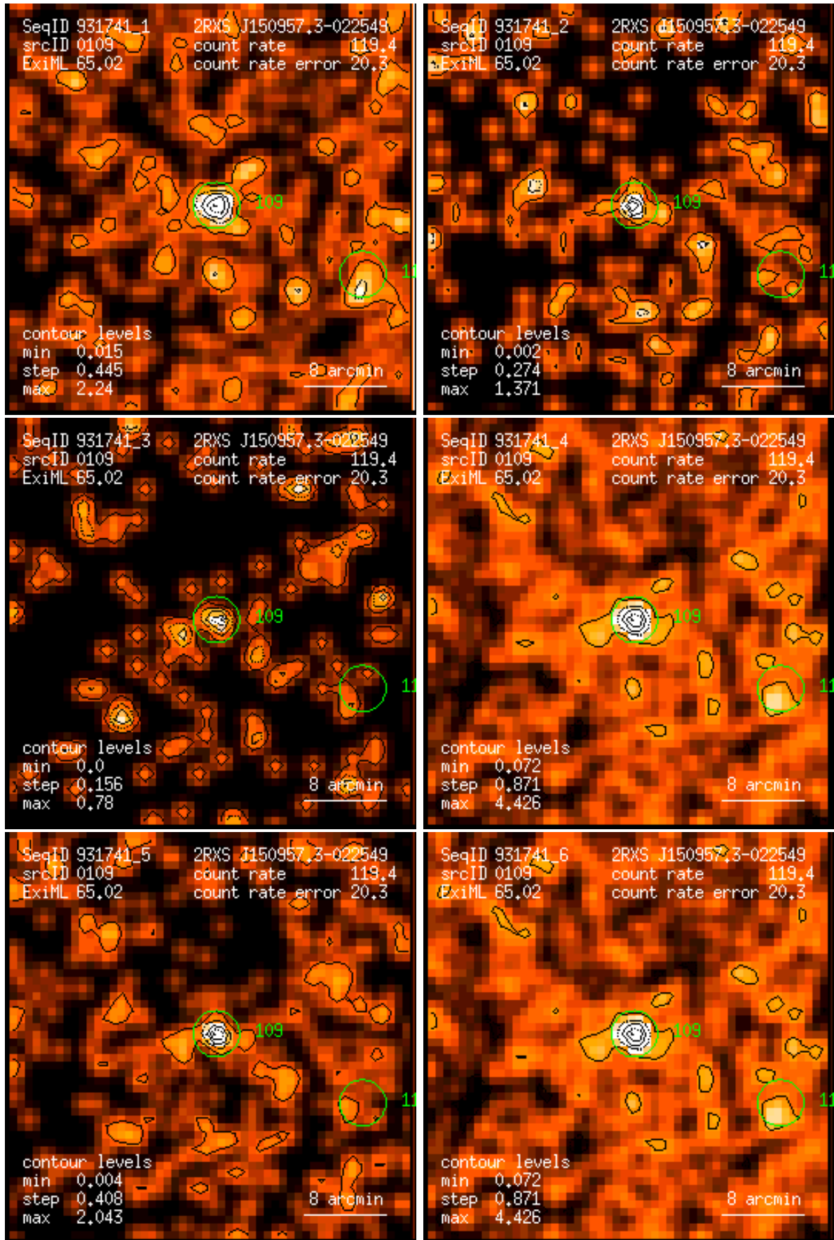
Figure 109: RASS 931741: detection 0109: band rate images, Gaussian filter: (1) PSPC channels 11 – 41, (2) 52 – 90, (3) 91 – 201, (4) 11 – 235, (5) 52 – 201, (6) 11 – 201. Broad band rates in counts/ks. Band rate contour levels in counts/ks/arcmin 2 .
