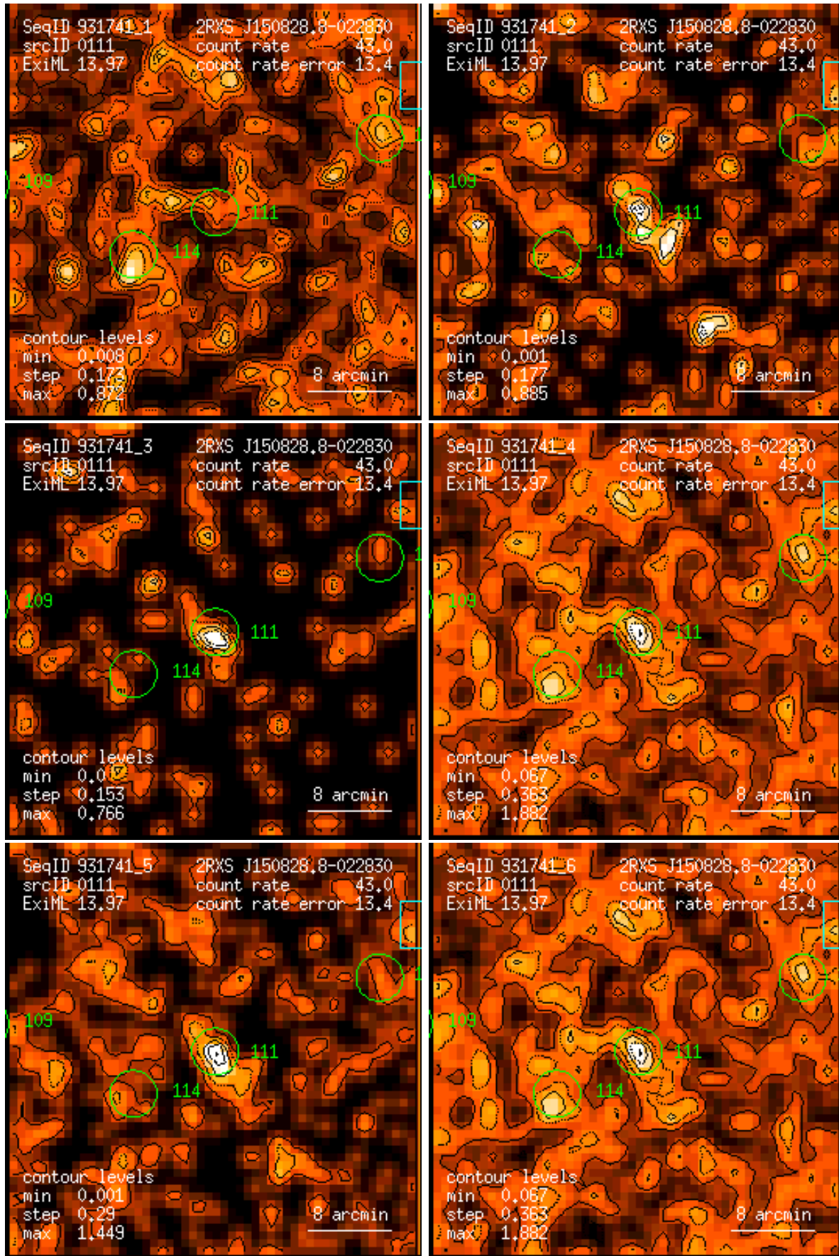
Figure 111: RASS 931741: detection 0111: band rate images, Gaussian filter: (1) PSPC channels 11 – 41, (2) 52 – 90, (3) 91 – 201, (4) 11 – 235, (5) 52 – 201, (6) 11 – 201. Broad band rates in counts/ks. Band rate contour levels in counts/ks/arcmin 2 .
