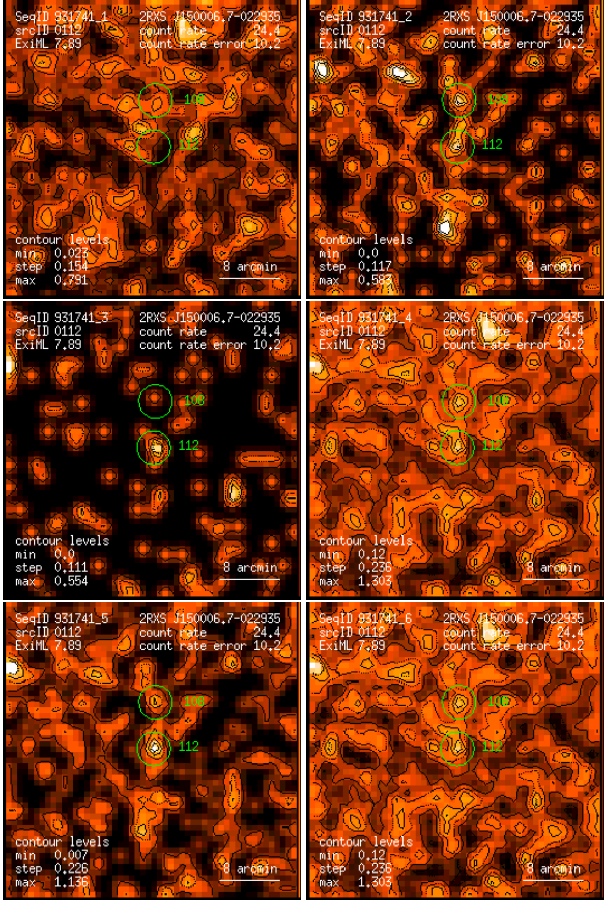
Figure 112: RASS 931741: detection 0112: band rate images, Gaussian filter: (1) PSPC channels 11 – 41, (2) 52 – 90, (3) 91 – 201, (4) 11 – 235, (5) 52 – 201, (6) 11 – 201. Broad band rates in counts/ks. Band rate contour levels in counts/ks/arcmin 2 .
