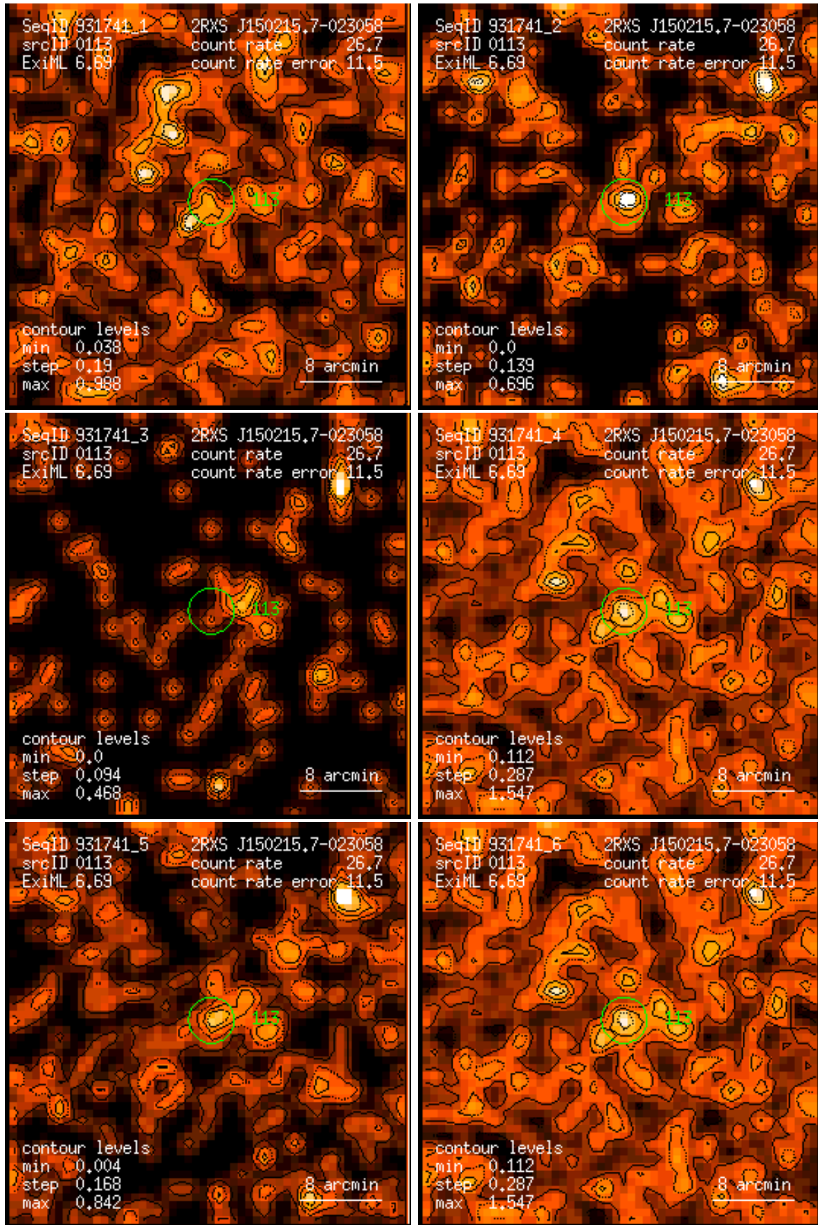
Figure 113: RASS 931741: detection 0113: band rate images, Gaussian filter: (1) PSPC channels 11 – 41, (2) 52 – 90, (3) 91 – 201, (4) 11 – 235, (5) 52 – 201, (6) 11 – 201. Broad band rates in counts/ks. Band rate contour levels in counts/ks/arcmin 2 .
