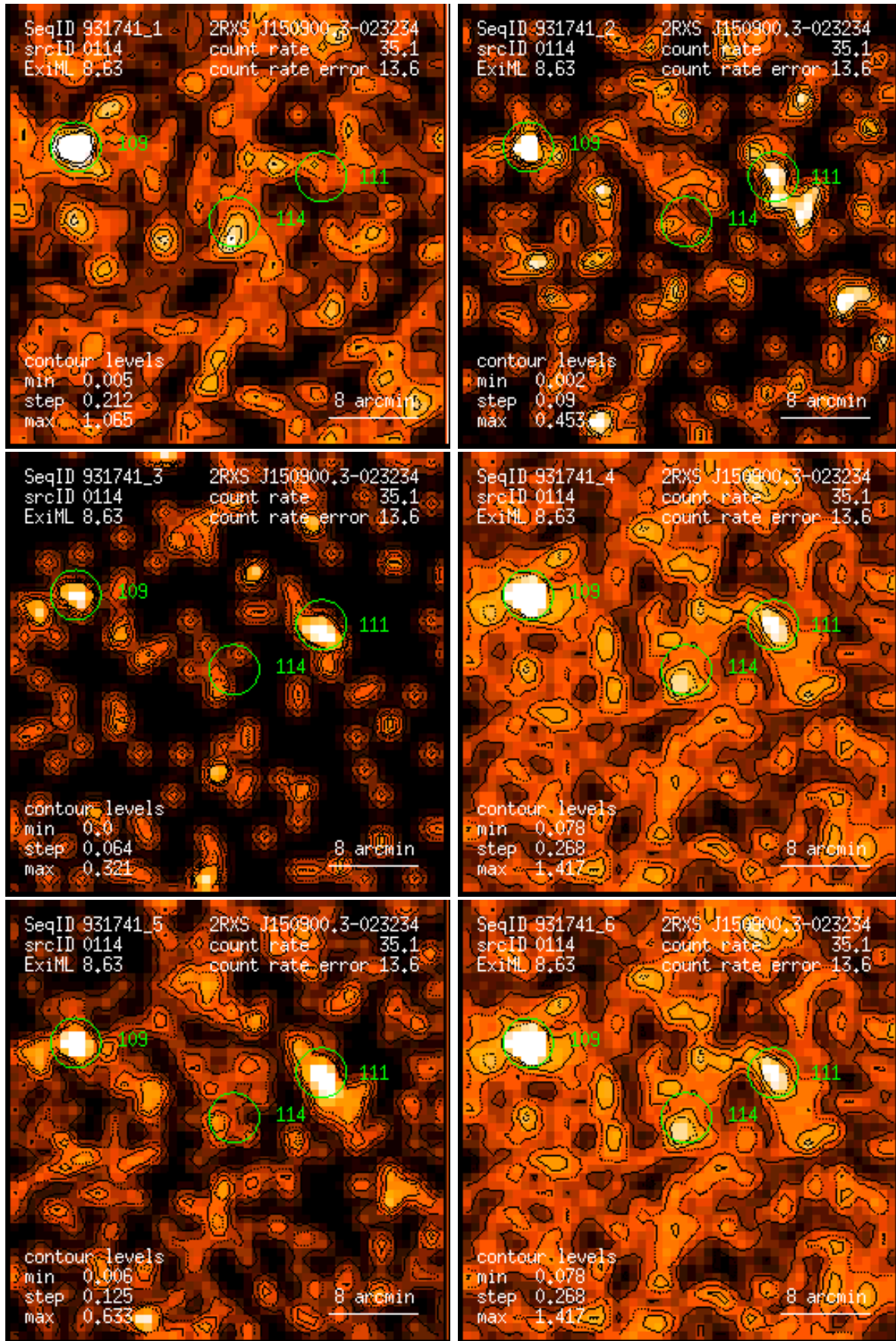
Figure 114: RASS 931741: detection 0114: band rate images, Gaussian filter: (1) PSPC channels 11 – 41, (2) 52 – 90, (3) 91 – 201, (4) 11 – 235, (5) 52 – 201, (6) 11 – 201. Broad band rates in counts/ks. Band rate contour levels in counts/ks/arcmin 2 .
