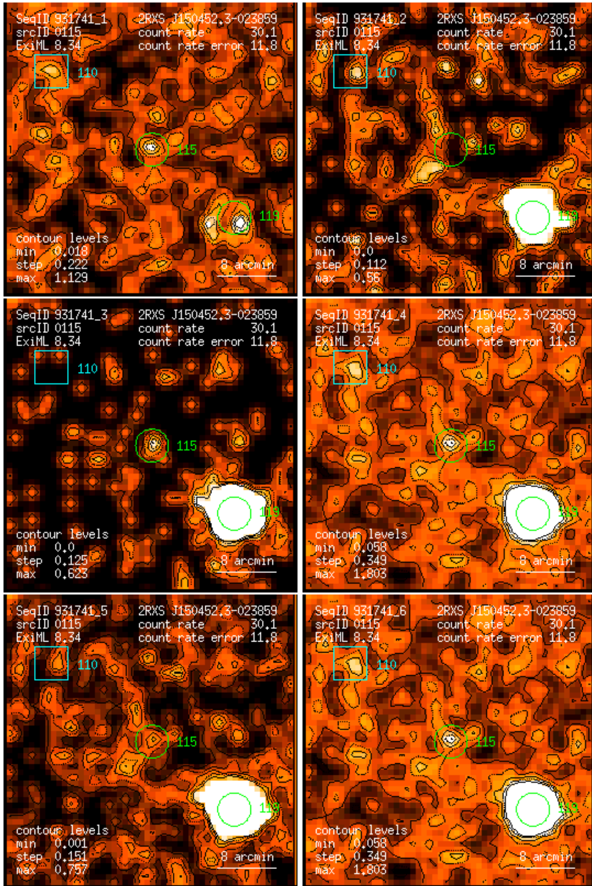
Figure 115: RASS 931741: detection 0115: band rate images, Gaussian filter: (1) PSPC channels 11 – 41, (2) 52 – 90, (3) 91 – 201, (4) 11 – 235, (5) 52 – 201, (6) 11 – 201. Broad band rates in counts/ks. Band rate contour levels in counts/ks/arcmin 2 .
