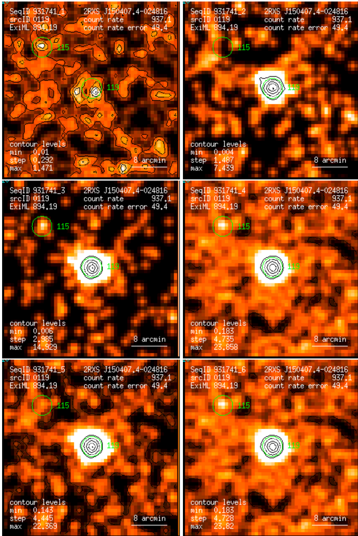
Figure 119: RASS 931741: detection 0119: band rate images, Gaussian filter: (1) PSPC channels 11 – 41, (2) 52 – 90, (3) 91 – 201, (4) 11 – 235, (5) 52 – 201, (6) 11 – 201. Broad band rates in counts/ks. Band rate contour levels in counts/ks/arcmin 2 .
