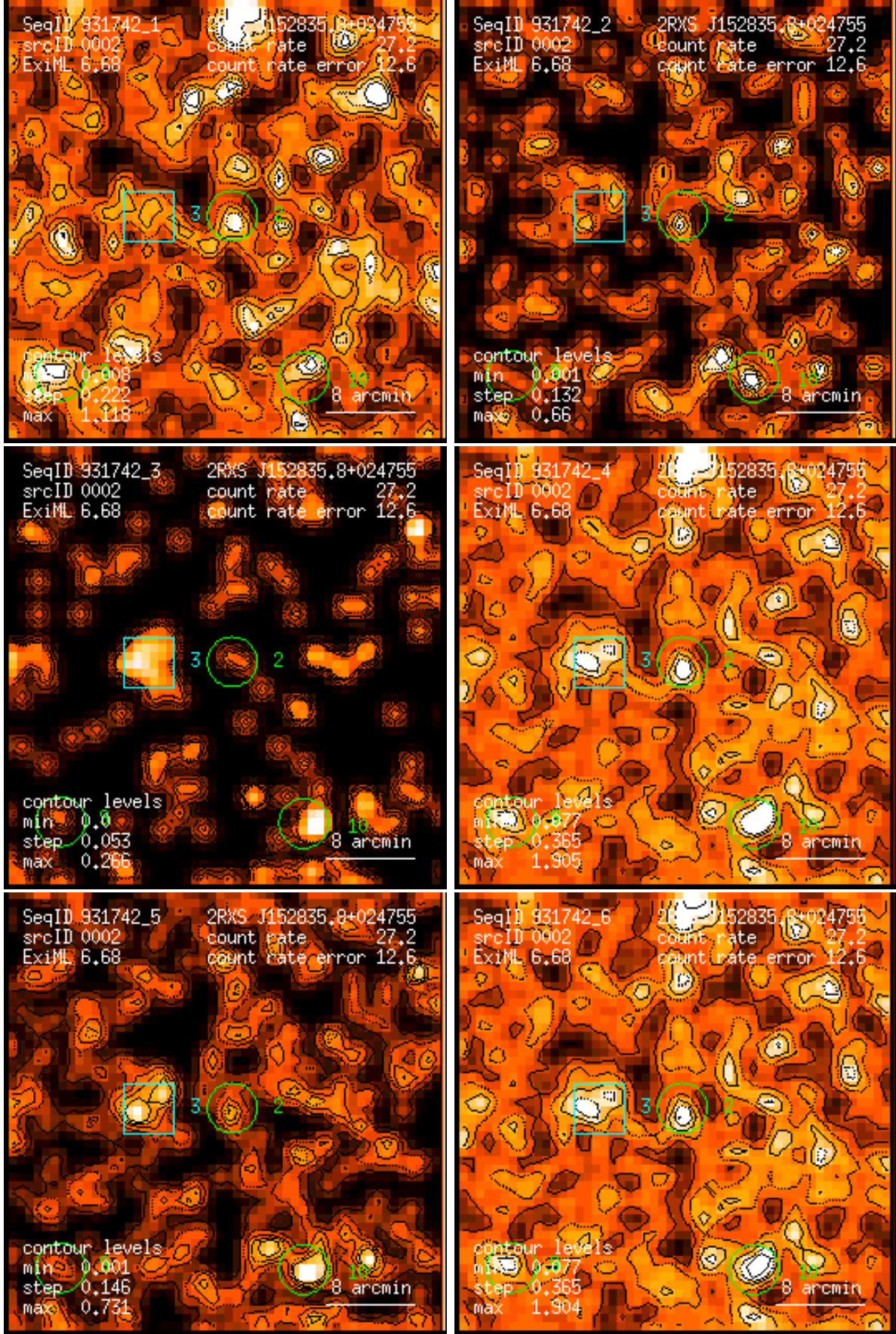
Figure 2: RASS 931742: detection 0002: band rate images, Gaussian filter: (1) PSPC channels 11 – 41, (2) 52 – 90, (3) 91 – 201, (4) 11 – 235, (5) 52 – 201, (6) 11 – 201. Broad band rates in counts/ks. Band rate contour levels in counts/ks/arcmin 2 .
