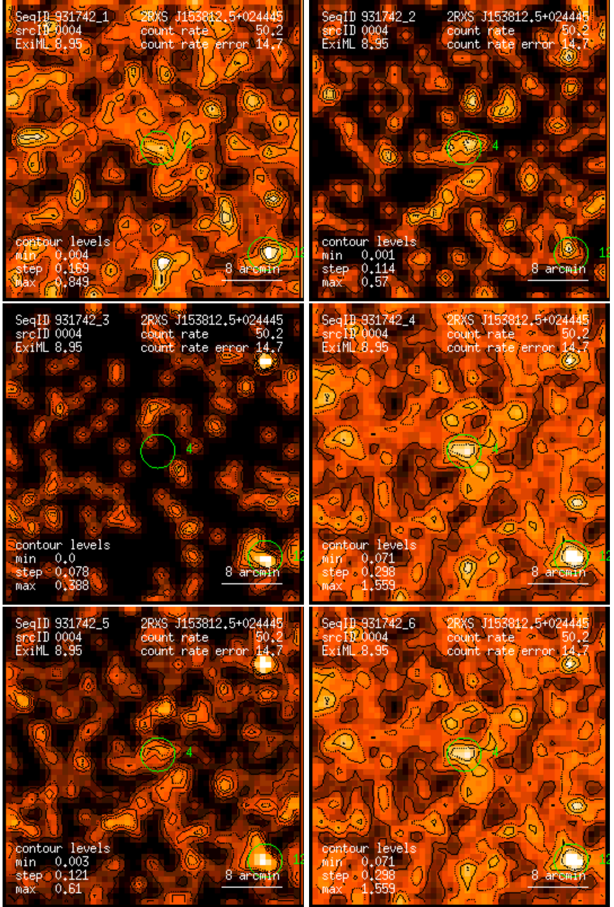
Figure 4: RASS 931742: detection 0004: band rate images, Gaussian filter: (1) PSPC channels 11 – 41, (2) 52 – 90, (3) 91 – 201, (4) 11 – 235, (5) 52 – 201, (6) 11 – 201. Broad band rates in counts/ks. Band rate contour levels in counts/ks/arcmin 2 .
