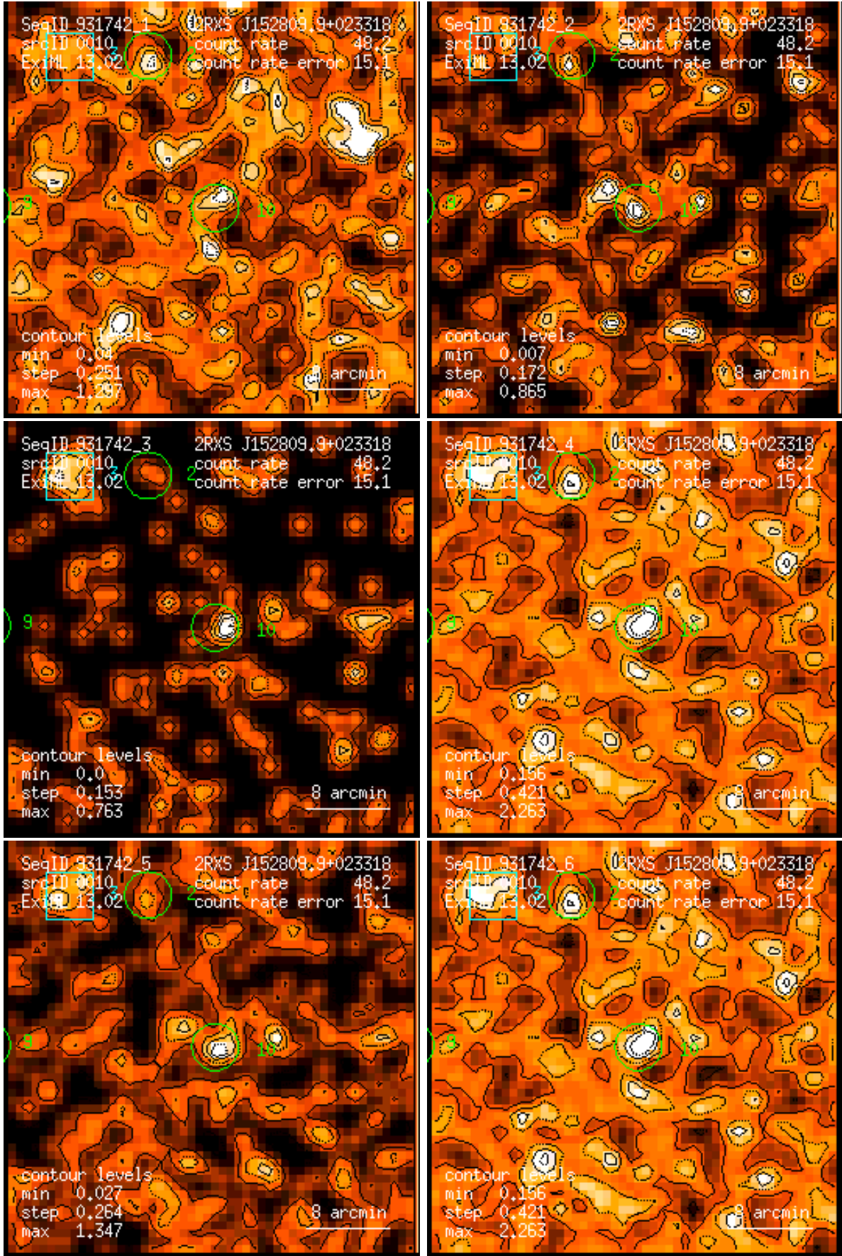
Figure 10: RASS 931742: detection 0010: band rate images, Gaussian filter: (1) PSPC channels 11 – 41, (2) 52 – 90, (3) 91 – 201, (4) 11 – 235, (5) 52 – 201, (6) 11 – 201. Broad band rates in counts/ks. Band rate contour levels in counts/ks/arcmin 2 .
