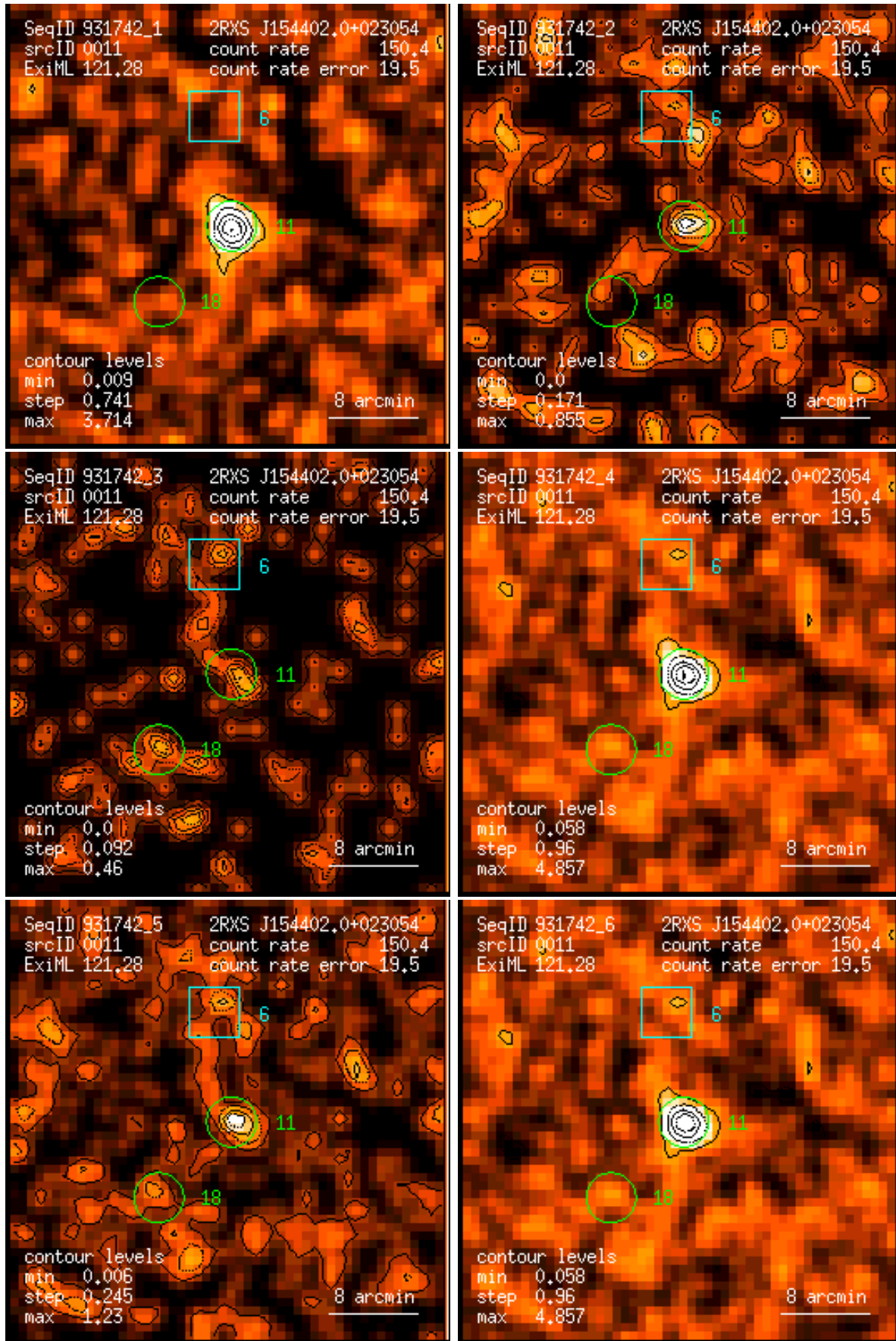
Figure 11: RASS 931742: detection 0011: band rate images, Gaussian filter: (1) PSPC channels 11 – 41, (2) 52 – 90, (3) 91 – 201, (4) 11 – 235, (5) 52 – 201, (6) 11 – 201. Broad band rates in counts/ks. Band rate contour levels in counts/ks/arcmin 2 .
