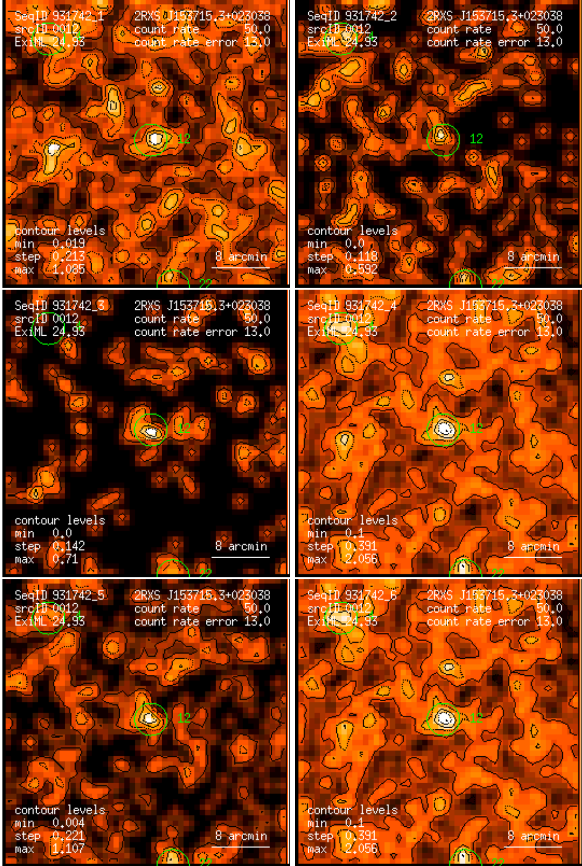
Figure 12: RASS 931742: detection 0012: band rate images, Gaussian filter: (1) PSPC channels 11 – 41, (2) 52 – 90, (3) 91 – 201, (4) 11 – 235, (5) 52 – 201, (6) 11 – 201. Broad band rates in counts/ks. Band rate contour levels in counts/ks/arcmin 2 .
