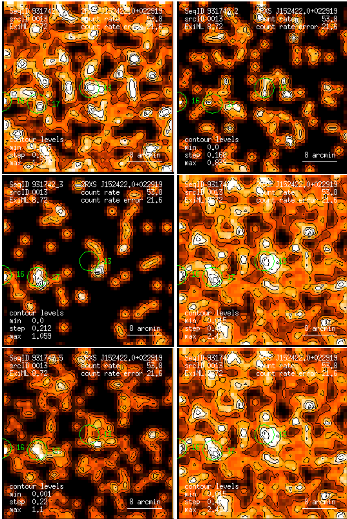
Figure 13: RASS 931742: detection 0013: band rate images, Gaussian filter: (1) PSPC channels 11 – 41, (2) 52 – 90, (3) 91 – 201, (4) 11 – 235, (5) 52 – 201, (6) 11 – 201. Broad band rates in counts/ks. Band rate contour levels in counts/ks/arcmin 2 .
