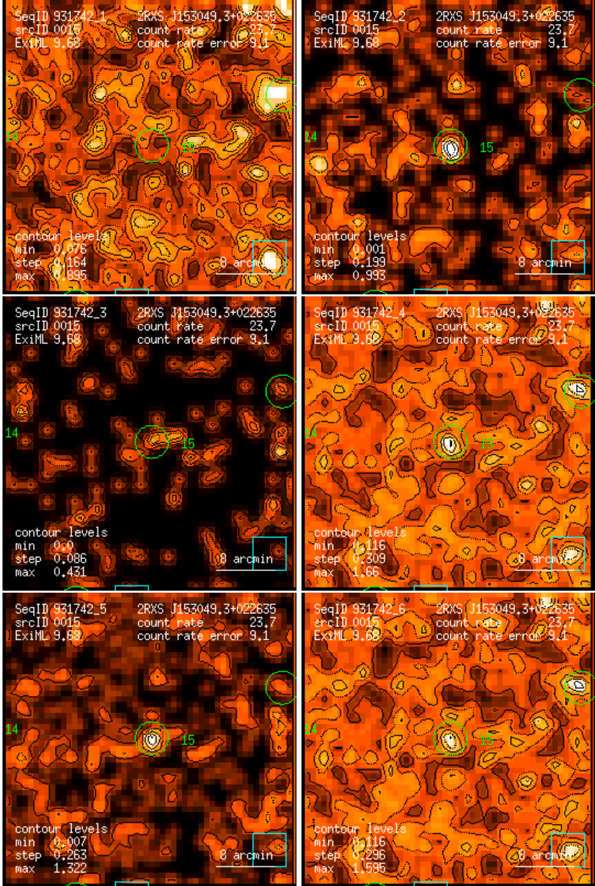
Figure 15: RASS 931742: detection 0015: band rate images, Gaussian filter: (1) PSPC channels 11 – 41, (2) 52 – 90, (3) 91 – 201, (4) 11 – 235, (5) 52 – 201, (6) 11 – 201. Broad band rates in counts/ks. Band rate contour levels in counts/ks/arcmin 2 .
