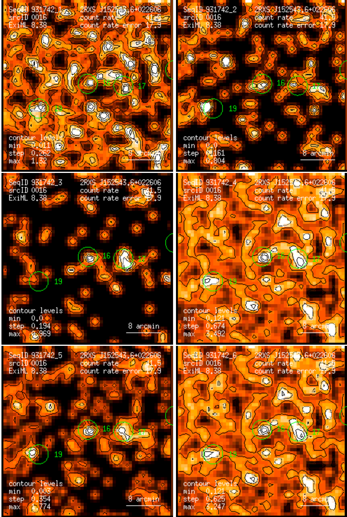
Figure 16: RASS 931742: detection 0016: band rate images, Gaussian filter: (1) PSPC channels 11 – 41, (2) 52 – 90, (3) 91 – 201, (4) 11 – 235, (5) 52 – 201, (6) 11 – 201. Broad band rates in counts/ks. Band rate contour levels in counts/ks/arcmin 2 .
