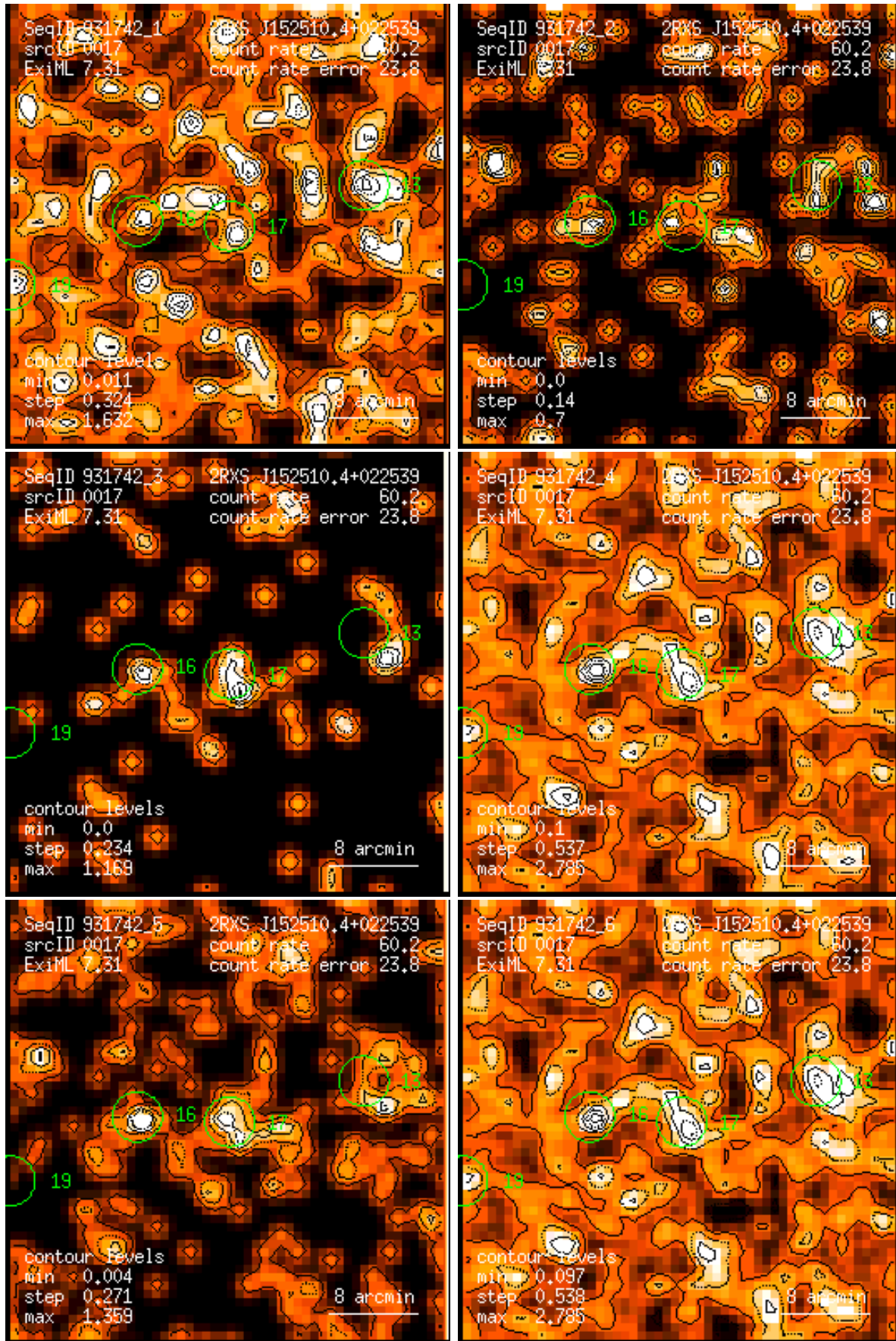
Figure 17: RASS 931742: detection 0017: band rate images, Gaussian filter: (1) PSPC channels 11 – 41, (2) 52 – 90, (3) 91 – 201, (4) 11 – 235, (5) 52 – 201, (6) 11 – 201. Broad band rates in counts/ks. Band rate contour levels in counts/ks/arcmin 2 .
