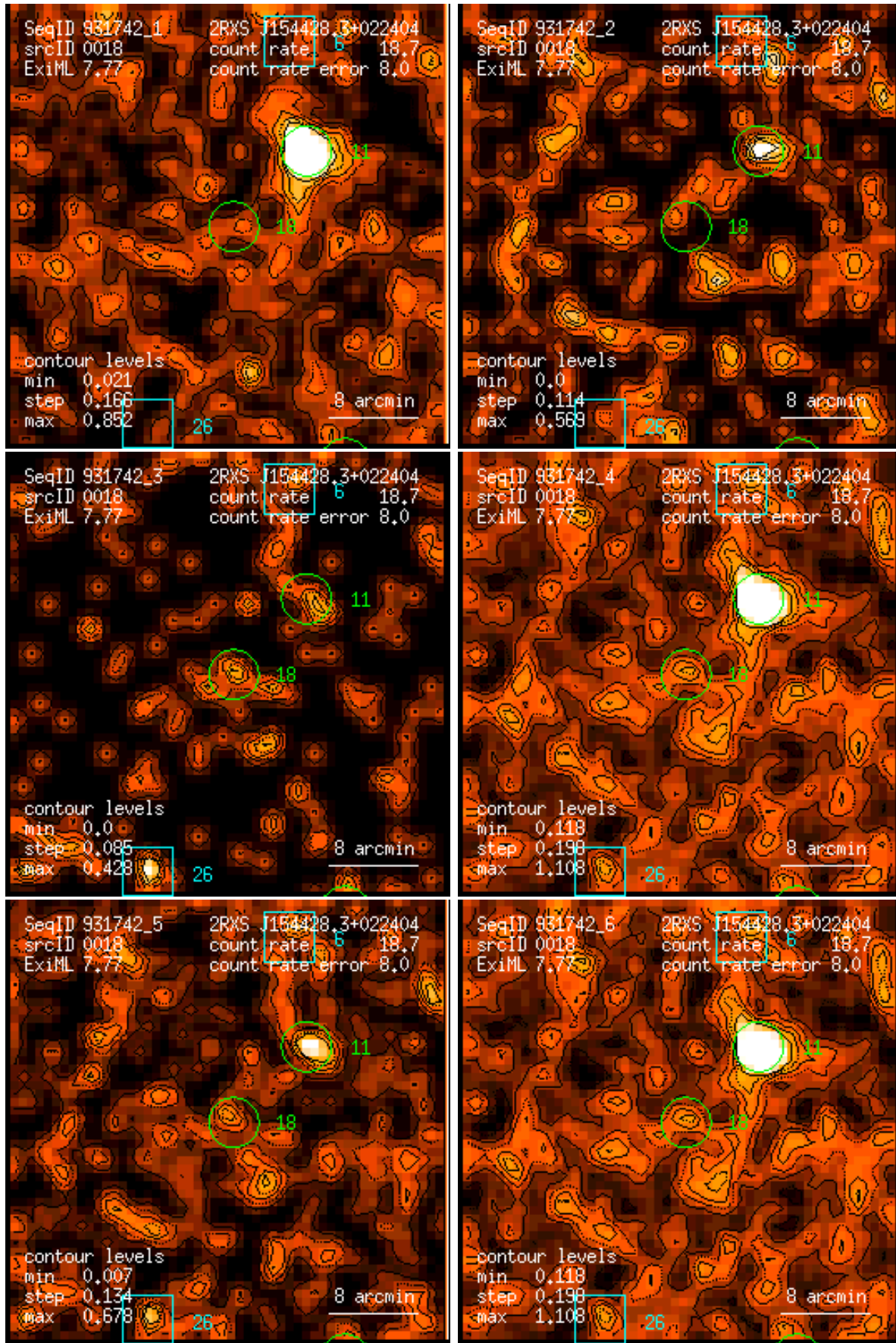
Figure 18: RASS 931742: detection 0018: band rate images, Gaussian filter: (1) PSPC channels 11 – 41, (2) 52 – 90, (3) 91 – 201, (4) 11 – 235, (5) 52 – 201, (6) 11 – 201. Broad band rates in counts/ks. Band rate contour levels in counts/ks/arcmin 2 .
