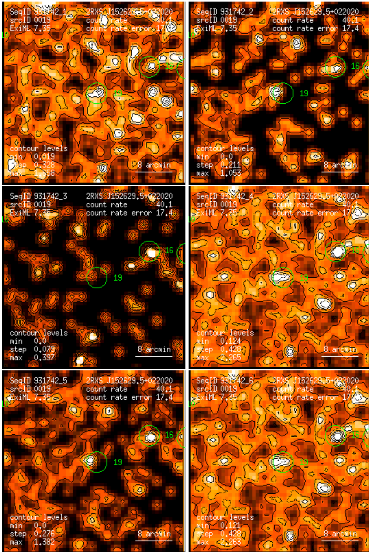
Figure 19: RASS 931742: detection 0019: band rate images, Gaussian filter: (1) PSPC channels 11 – 41, (2) 52 – 90, (3) 91 – 201, (4) 11 – 235, (5) 52 – 201, (6) 11 – 201. Broad band rates in counts/ks. Band rate contour levels in counts/ks/arcmin 2 .
