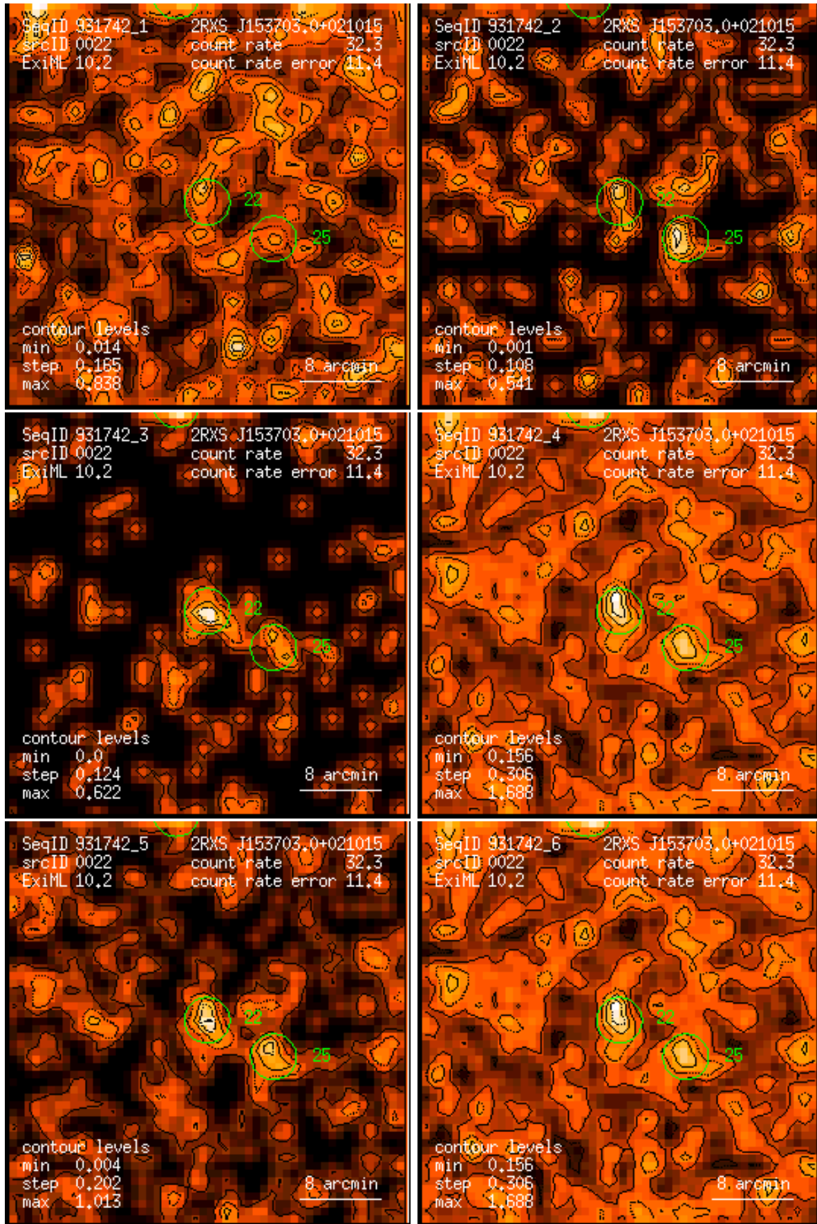
Figure 22: RASS 931742: detection 0022: band rate images, Gaussian filter: (1) PSPC channels 11 – 41, (2) 52 – 90, (3) 91 – 201, (4) 11 – 235, (5) 52 – 201, (6) 11 – 201. Broad band rates in counts/ks. Band rate contour levels in counts/ks/arcmin 2 .
