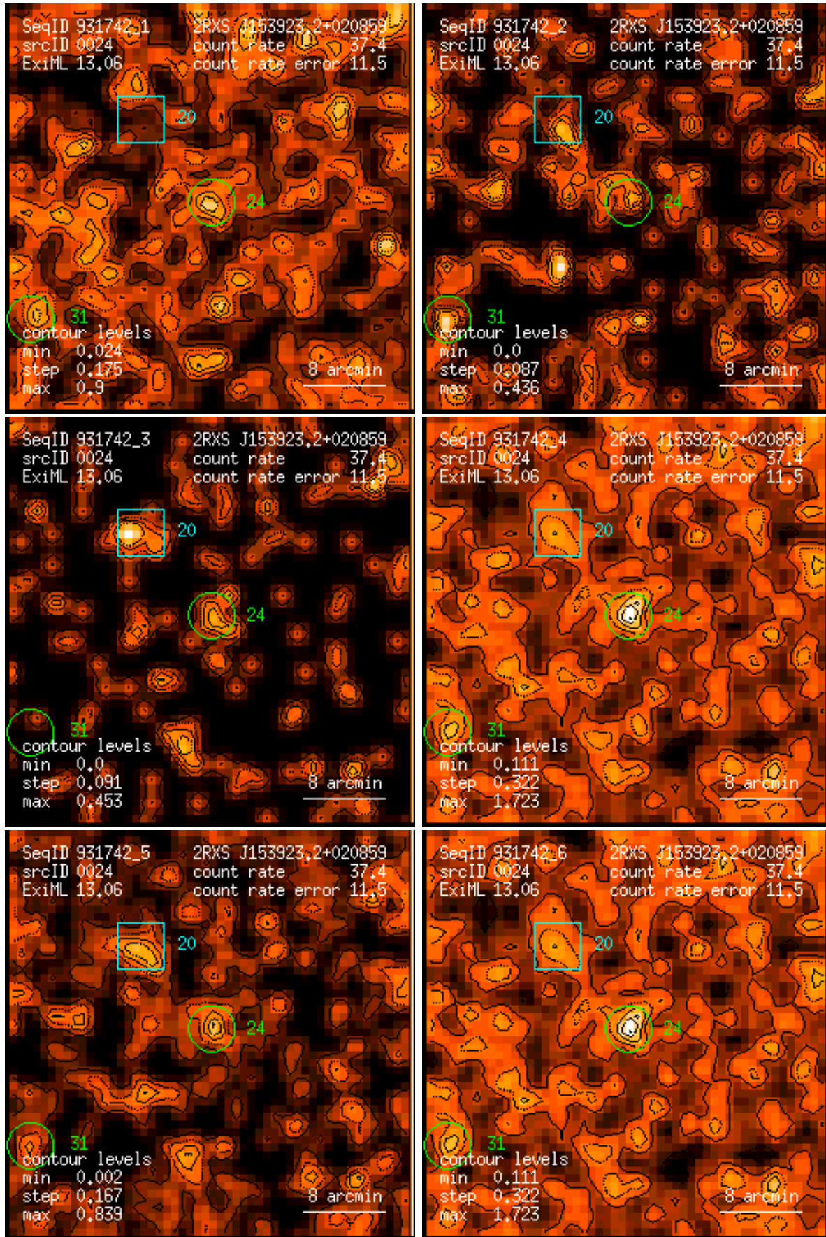
Figure 24: RASS 931742: detection 0024: band rate images, Gaussian filter: (1) PSPC channels 11 – 41, (2) 52 – 90, (3) 91 – 201, (4) 11 – 235, (5) 52 – 201, (6) 11 – 201. Broad band rates in counts/ks. Band rate contour levels in counts/ks/arcmin 2 .
