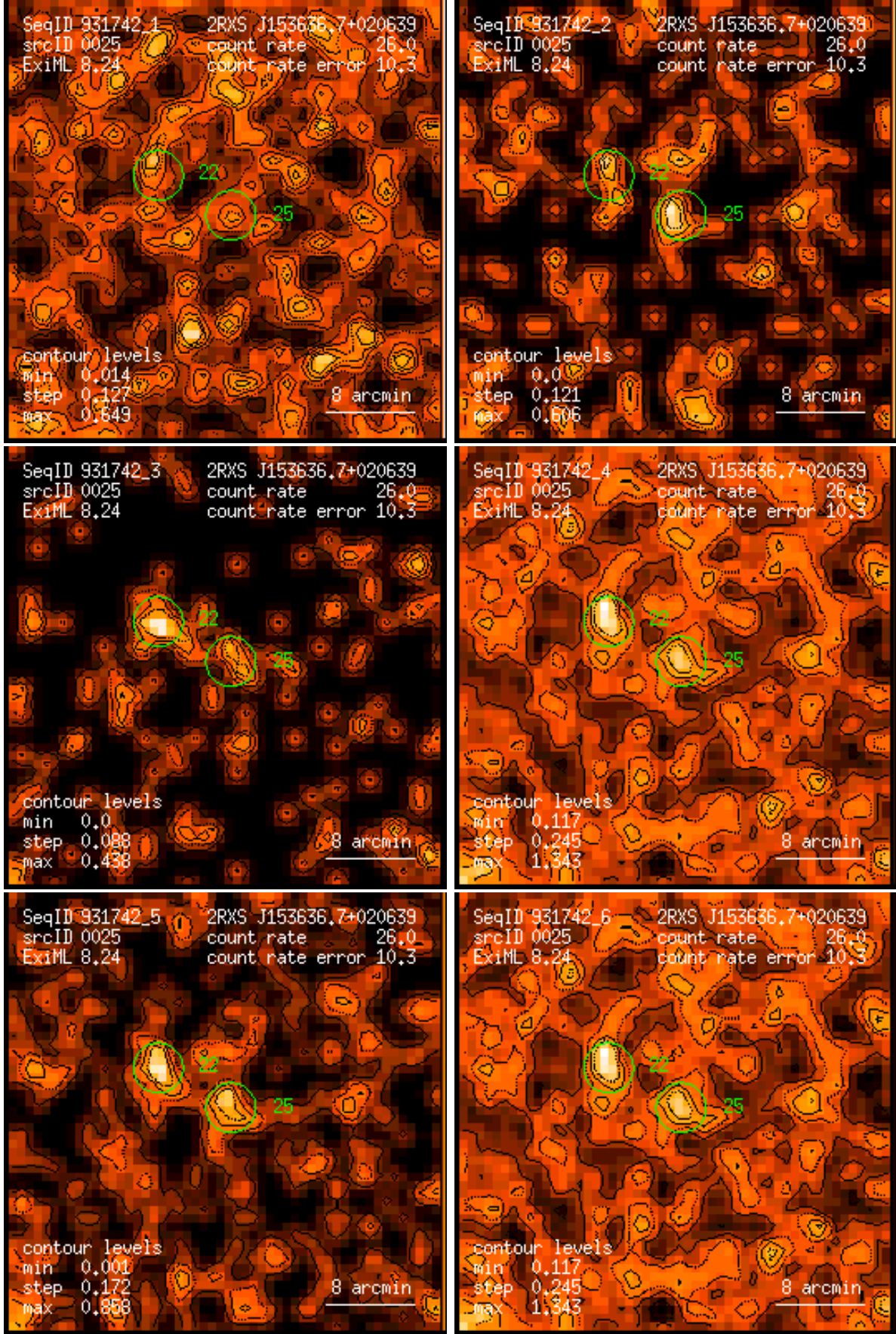
Figure 25: RASS 931742: detection 0025: band rate images, Gaussian filter: (1) PSPC channels 11 – 41, (2) 52 – 90, (3) 91 – 201, (4) 11 – 235, (5) 52 – 201, (6) 11 – 201. Broad band rates in counts/ks. Band rate contour levels in counts/ks/arcmin 2 .
