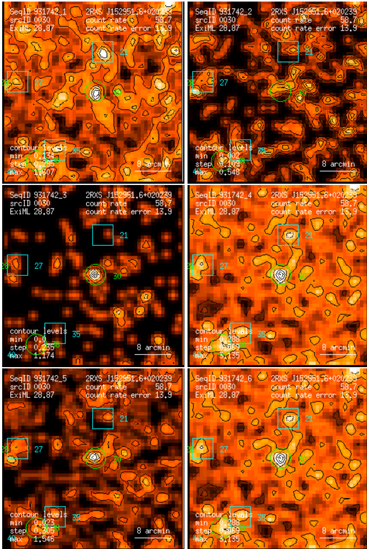
Figure 30: RASS 931742: detection 0030: band rate images, Gaussian filter: (1) PSPC channels 11 – 41, (2) 52 – 90, (3) 91 – 201, (4) 11 – 235, (5) 52 – 201, (6) 11 – 201. Broad band rates in counts/ks. Band rate contour levels in counts/ks/arcmin 2 .
