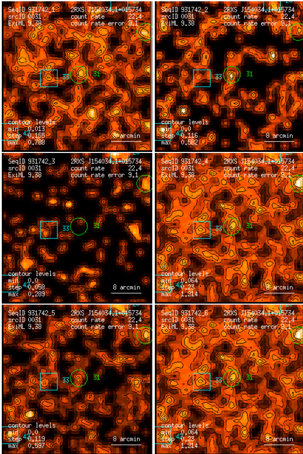
Figure 31: RASS 931742: detection 0031: band rate images, Gaussian filter: (1) PSPC channels 11 – 41, (2) 52 – 90, (3) 91 – 201, (4) 11 – 235, (5) 52 – 201, (6) 11 – 201. Broad band rates in counts/ks. Band rate contour levels in counts/ks/arcmin 2 .
