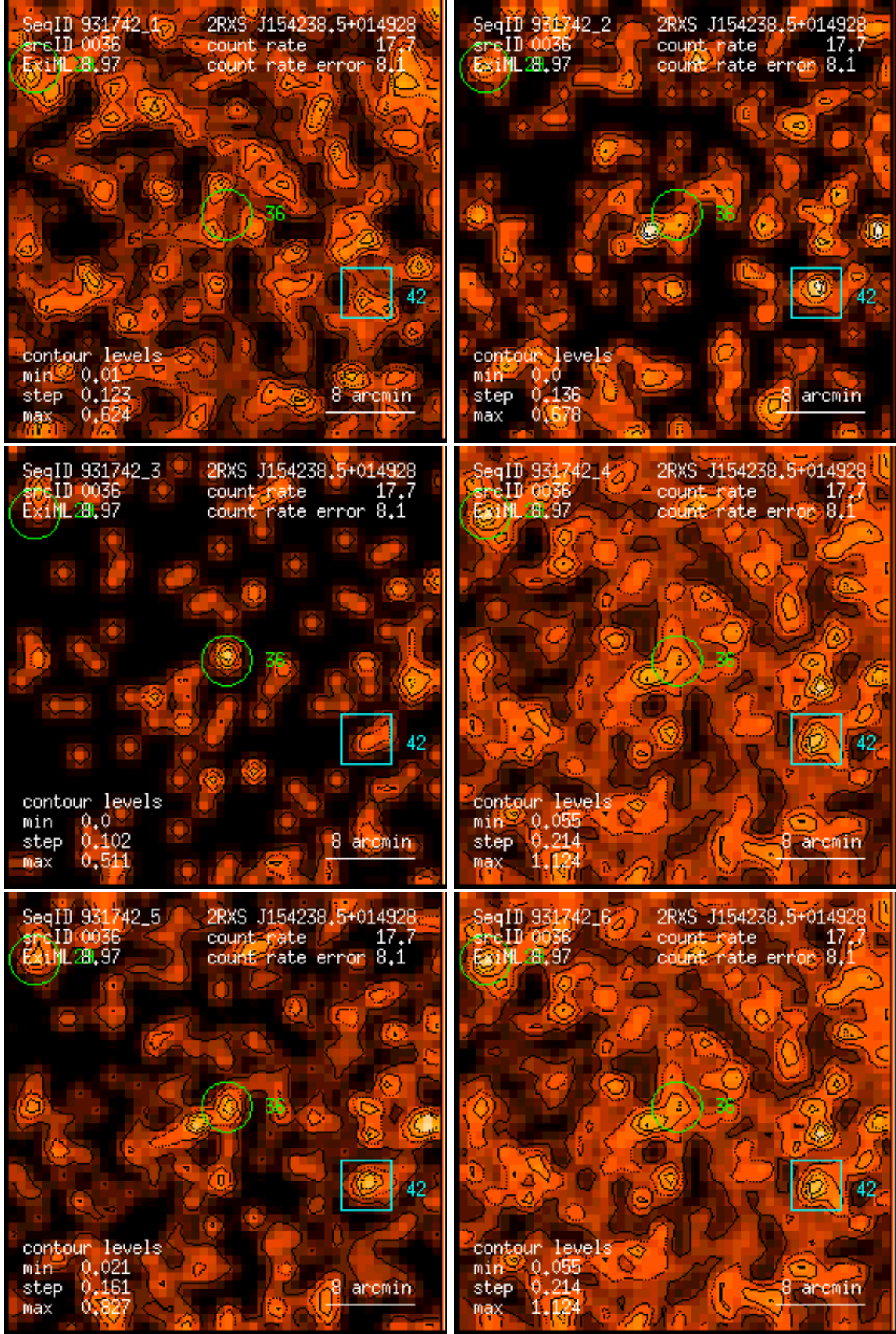
Figure 36: RASS 931742: detection 0036: band rate images, Gaussian filter: (1) PSPC channels 11 – 41, (2) 52 – 90, (3) 91 – 201, (4) 11 – 235, (5) 52 – 201, (6) 11 – 201. Broad band rates in counts/ks. Band rate contour levels in counts/ks/arcmin 2 .
