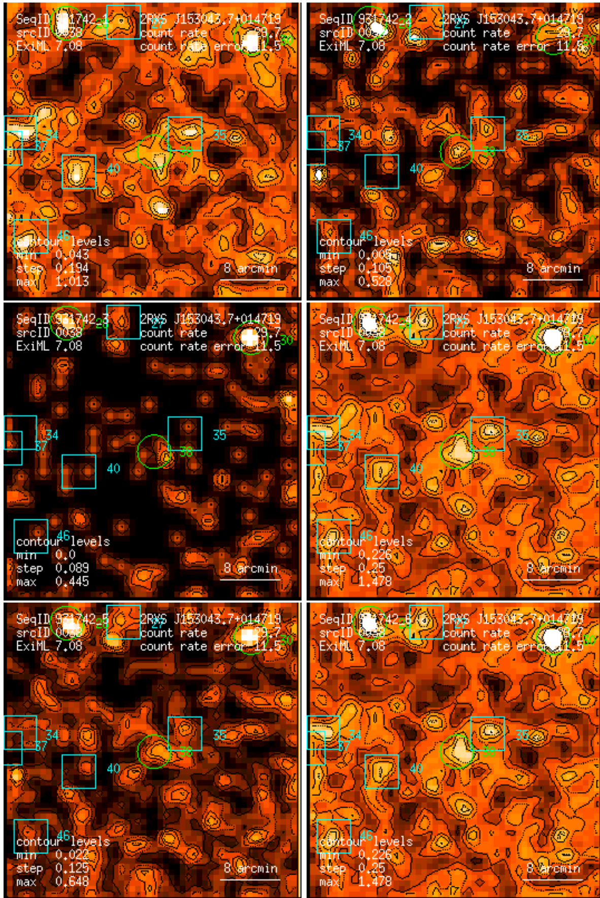
Figure 38: RASS 931742: detection 0038: band rate images, Gaussian filter: (1) PSPC channels 11 – 41, (2) 52 – 90, (3) 91 – 201, (4) 11 – 235, (5) 52 – 201, (6) 11 – 201. Broad band rates in counts/ks. Band rate contour levels in counts/ks/arcmin 2 .
