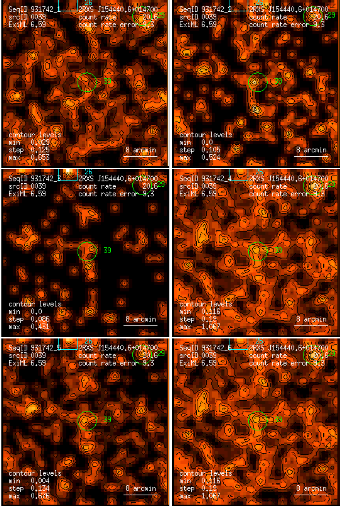
Figure 39: RASS 931742: detection 0039: band rate images, Gaussian filter: (1) PSPC channels 11 – 41, (2) 52 – 90, (3) 91 – 201, (4) 11 – 235, (5) 52 – 201, (6) 11 – 201. Broad band rates in counts/ks. Band rate contour levels in counts/ks/arcmin 2 .
