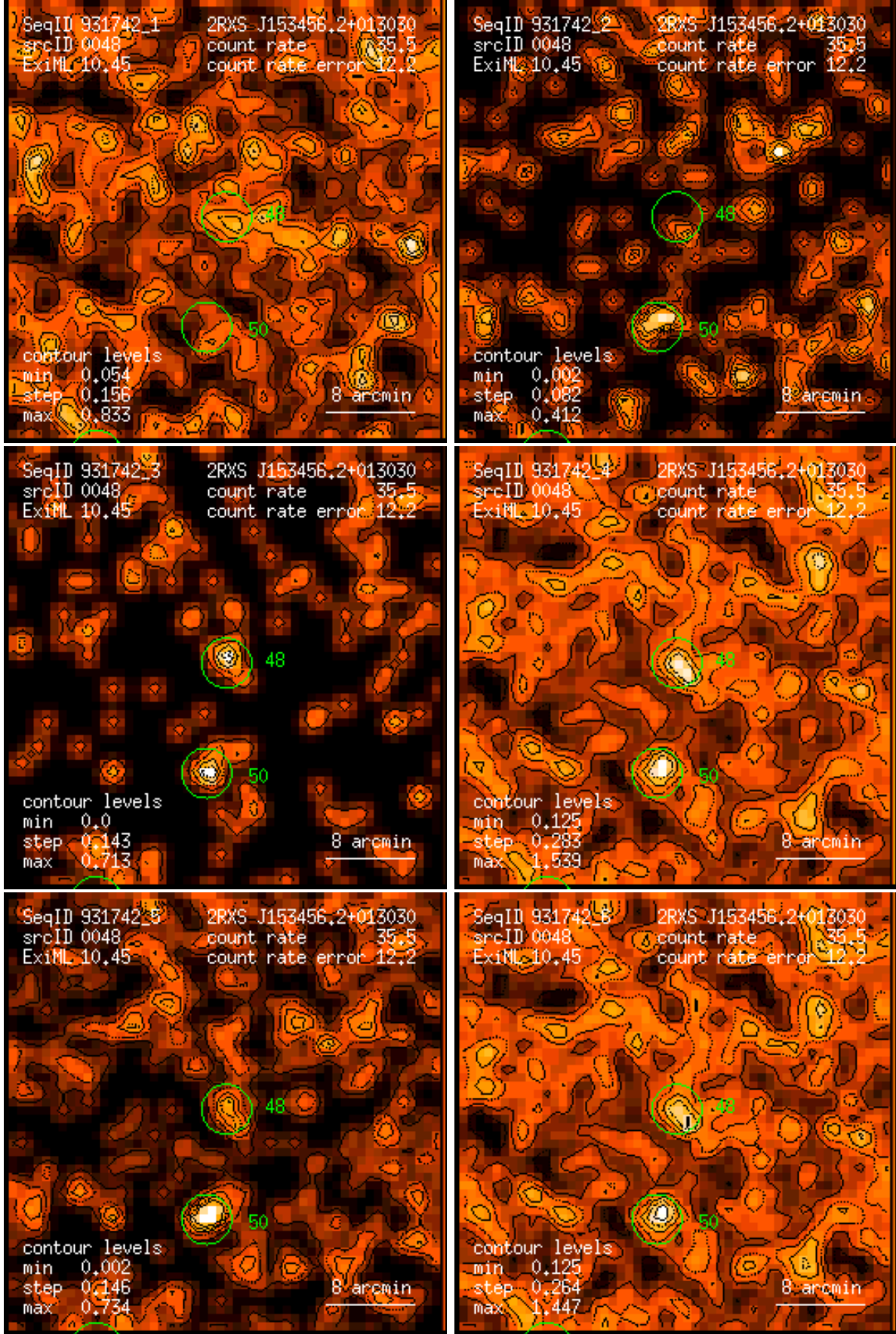
Figure 48: RASS 931742: detection 0048: band rate images, Gaussian filter: (1) PSPC channels 11 – 41, (2) 52 – 90, (3) 91 – 201, (4) 11 – 235, (5) 52 – 201, (6) 11 – 201. Broad band rates in counts/ks. Band rate contour levels in counts/ks/arcmin 2 .
