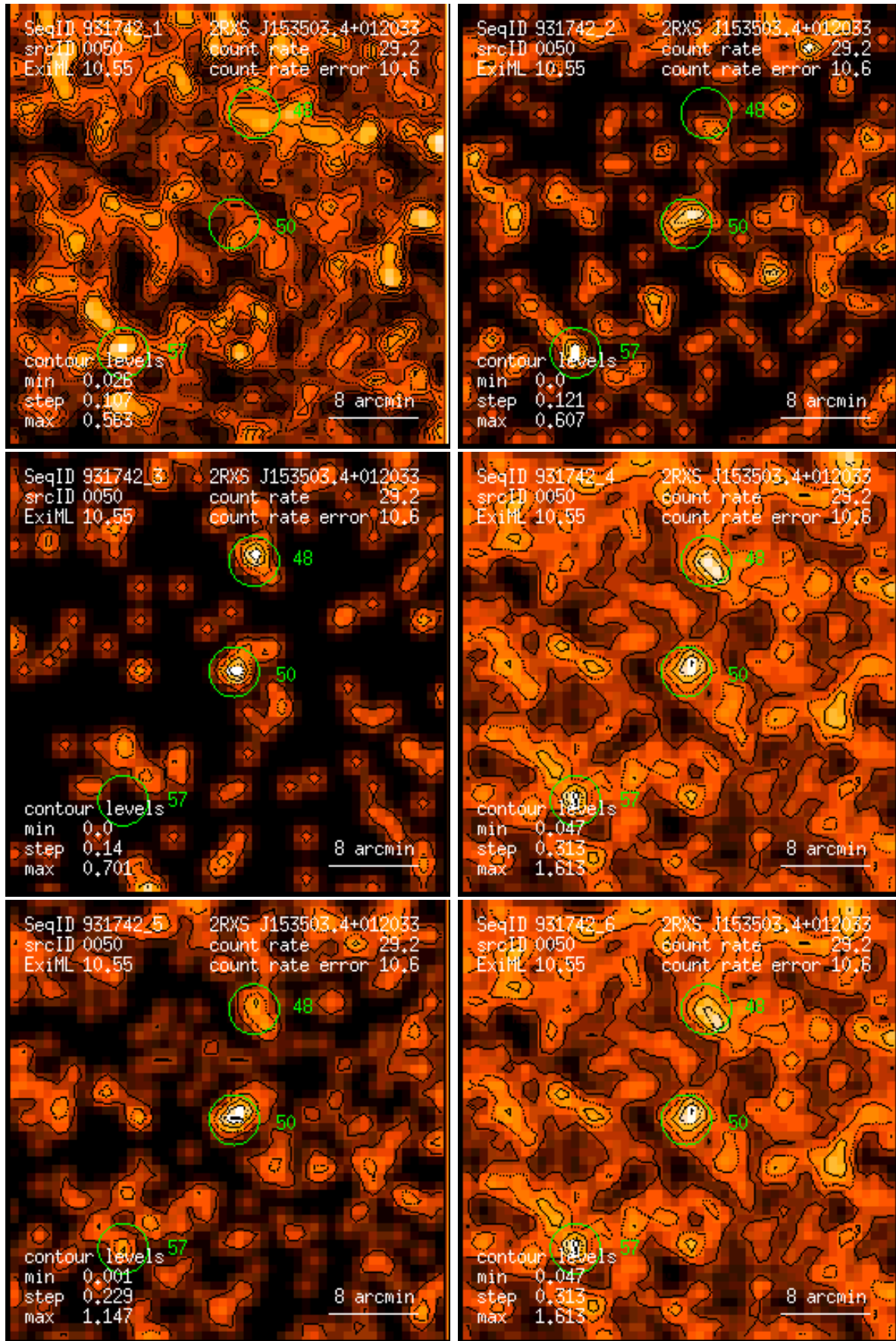
Figure 50: RASS 931742: detection 0050: band rate images, Gaussian filter: (1) PSPC channels 11 – 41, (2) 52 – 90, (3) 91 – 201, (4) 11 – 235, (5) 52 – 201, (6) 11 – 201. Broad band rates in counts/ks. Band rate contour levels in counts/ks/arcmin 2 .
