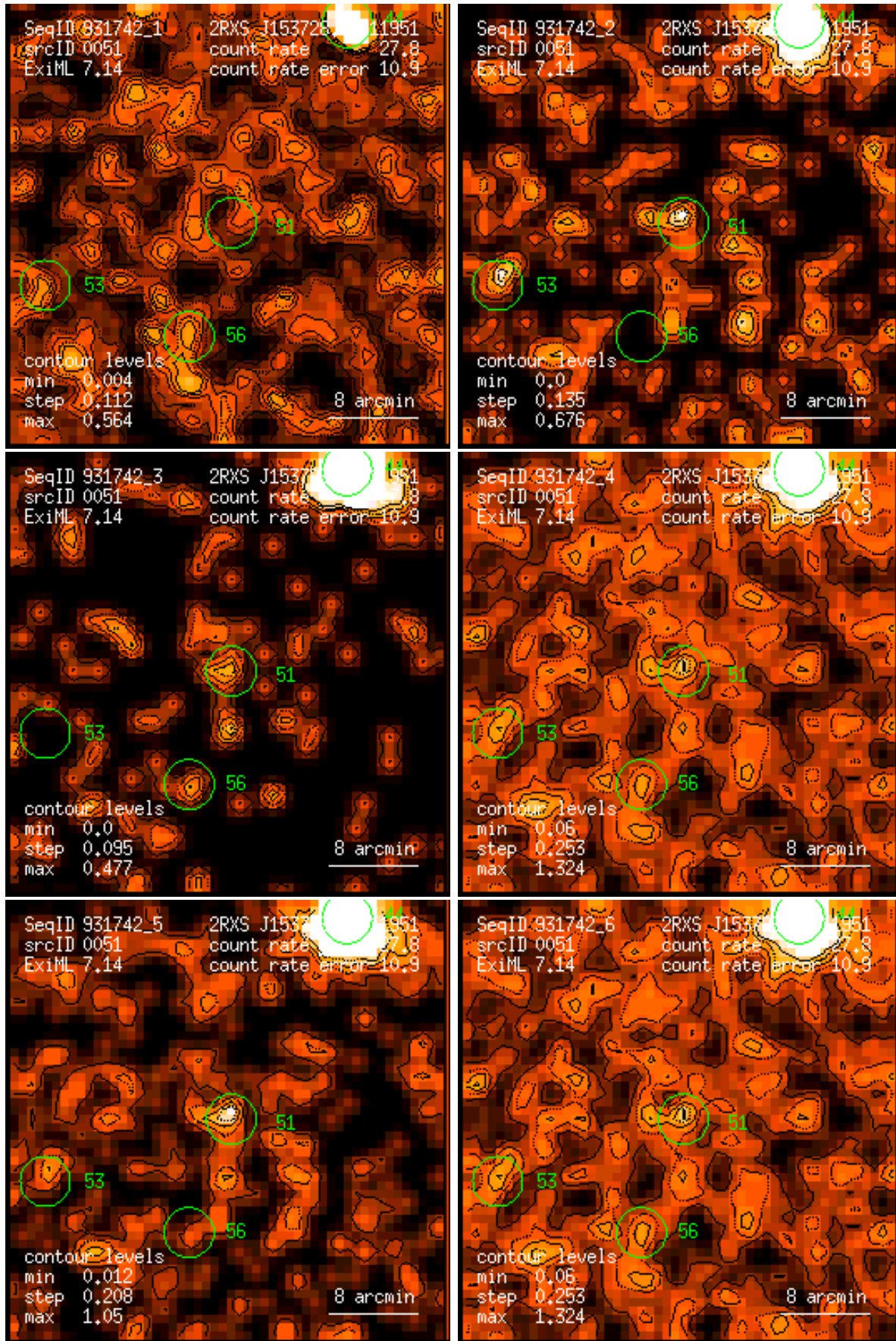
Figure 51: RASS 931742: detection 0051: band rate images, Gaussian filter: (1) PSPC channels 11 – 41, (2) 52 – 90, (3) 91 – 201, (4) 11 – 235, (5) 52 – 201, (6) 11 – 201. Broad band rates in counts/ks. Band rate contour levels in counts/ks/arcmin 2 .
