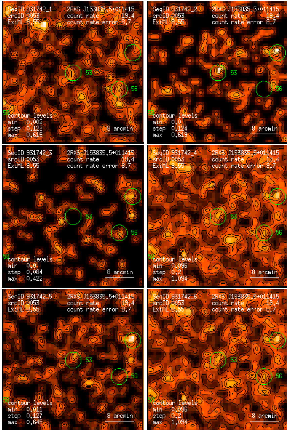
Figure 53: RASS 931742: detection 0053: band rate images, Gaussian filter: (1) PSPC channels 11 – 41, (2) 52 – 90, (3) 91 – 201, (4) 11 – 235, (5) 52 – 201, (6) 11 – 201. Broad band rates in counts/ks. Band rate contour levels in counts/ks/arcmin 2 .
