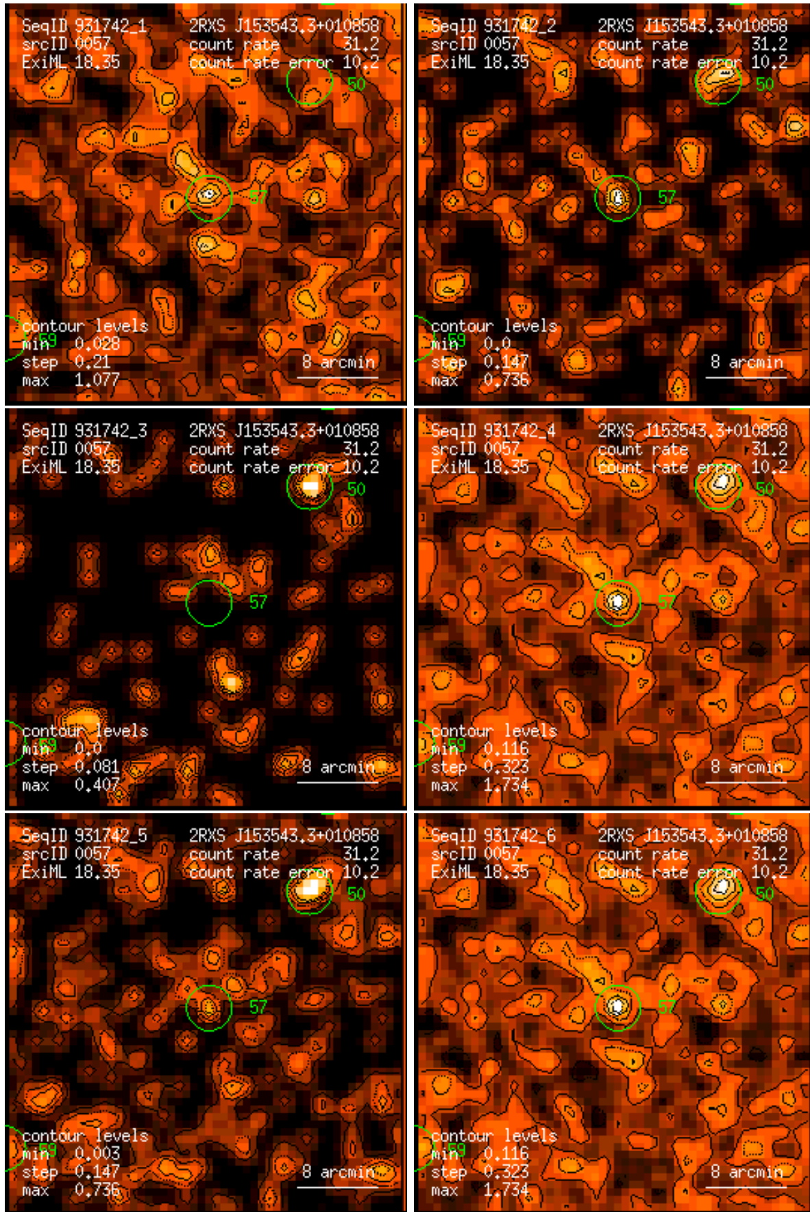
Figure 57: RASS 931742: detection 0057: band rate images, Gaussian filter: (1) PSPC channels 11 – 41, (2) 52 – 90, (3) 91 – 201, (4) 11 – 235, (5) 52 – 201, (6) 11 – 201. Broad band rates in counts/ks. Band rate contour levels in counts/ks/arcmin 2 .
