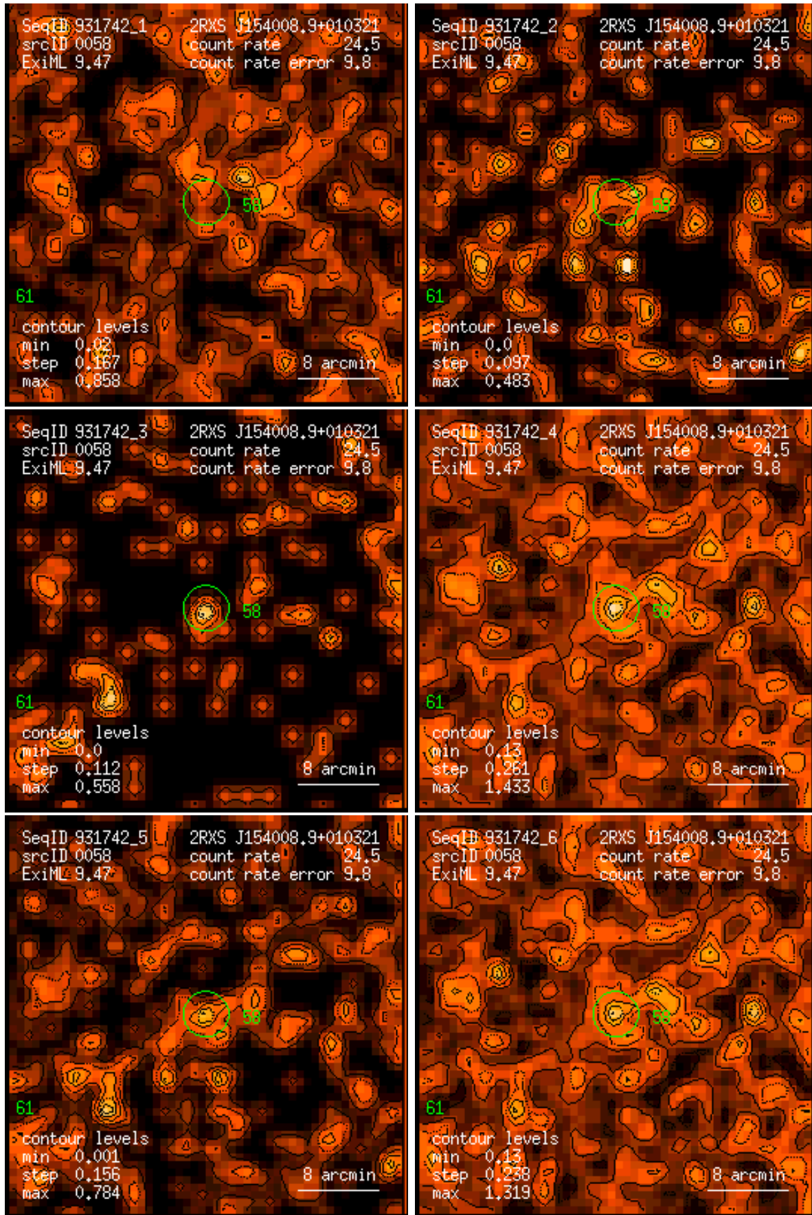
Figure 58: RASS 931742: detection 0058: band rate images, Gaussian filter: (1) PSPC channels 11 – 41, (2) 52 – 90, (3) 91 – 201, (4) 11 – 235, (5) 52 – 201, (6) 11 – 201. Broad band rates in counts/ks. Band rate contour levels in counts/ks/arcmin 2 .
