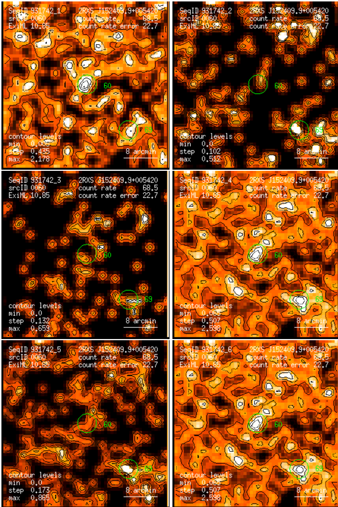
Figure 60: RASS 931742: detection 0060: band rate images, Gaussian filter: (1) PSPC channels 11 – 41, (2) 52 – 90, (3) 91 – 201, (4) 11 – 235, (5) 52 – 201, (6) 11 – 201. Broad band rates in counts/ks. Band rate contour levels in counts/ks/arcmin 2 .
