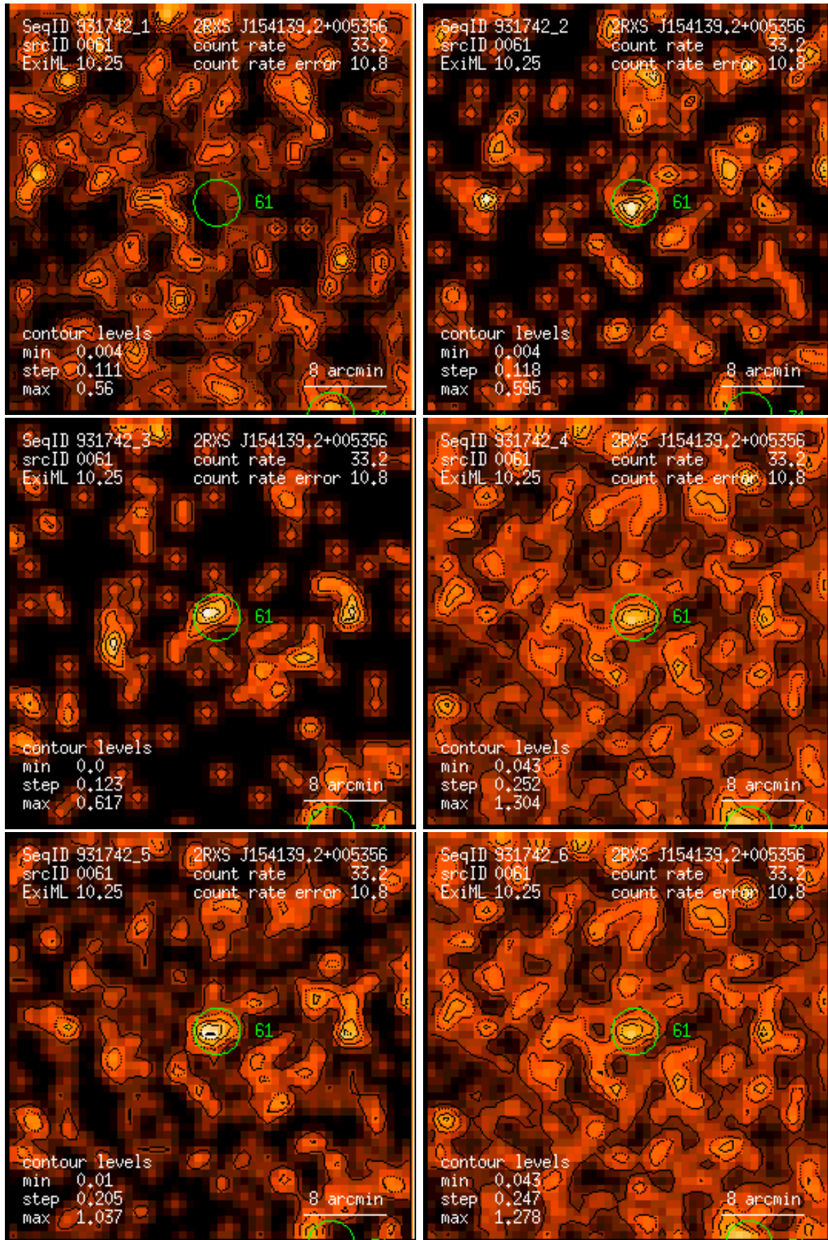
Figure 61: RASS 931742: detection 0061: band rate images, Gaussian filter: (1) PSPC channels 11 – 41, (2) 52 – 90, (3) 91 – 201, (4) 11 – 235, (5) 52 – 201, (6) 11 – 201. Broad band rates in counts/ks. Band rate contour levels in counts/ks/arcmin 2 .
